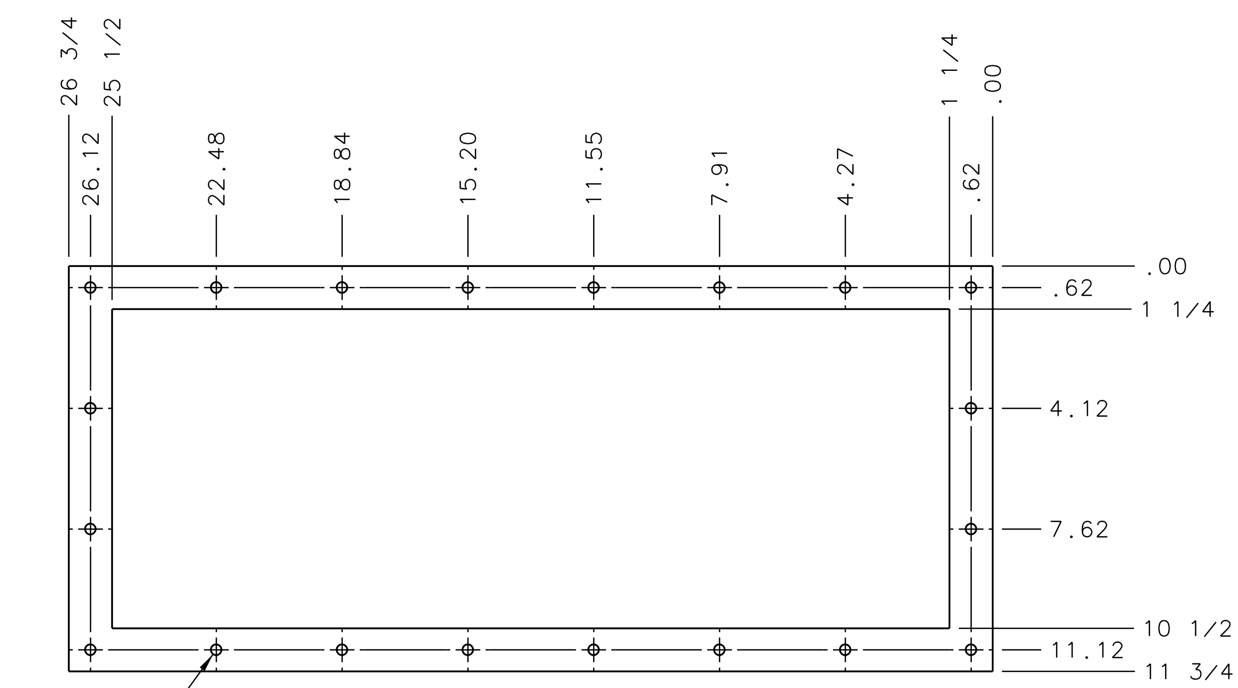
-04 ACCESS COVER SEAL
