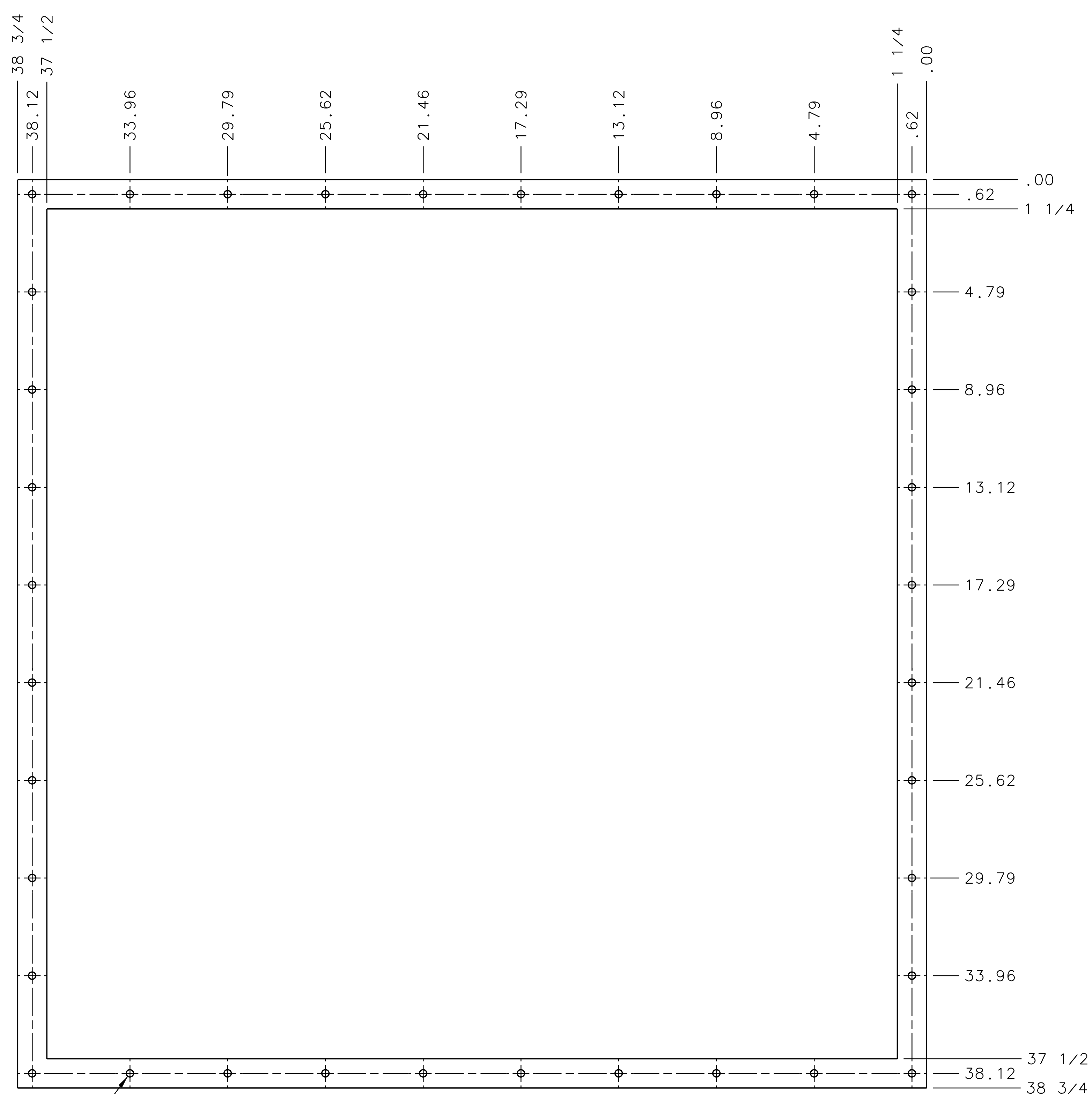
-01 REAR SEAL
