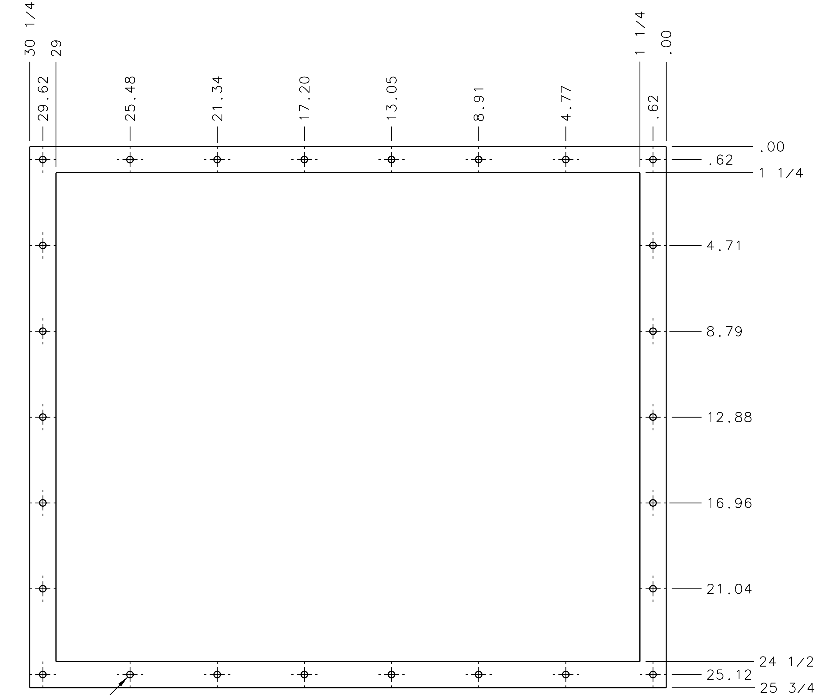
-02 FRONT SEAL
