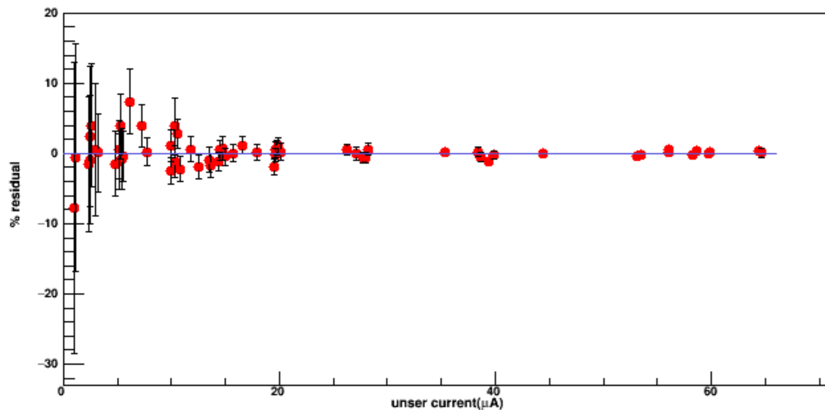
% Residual vs Unser Current
