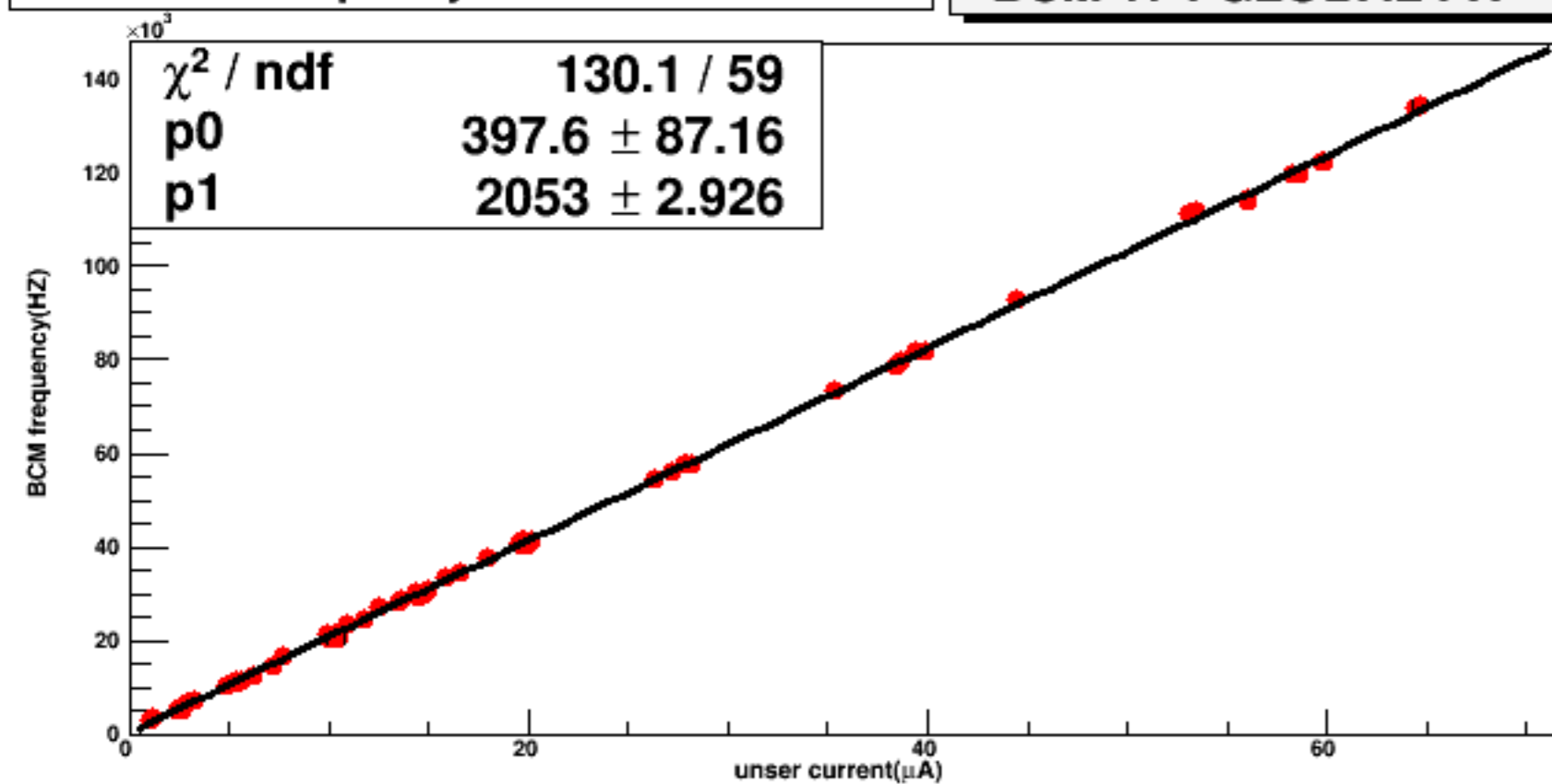
Frequency vs Unser
