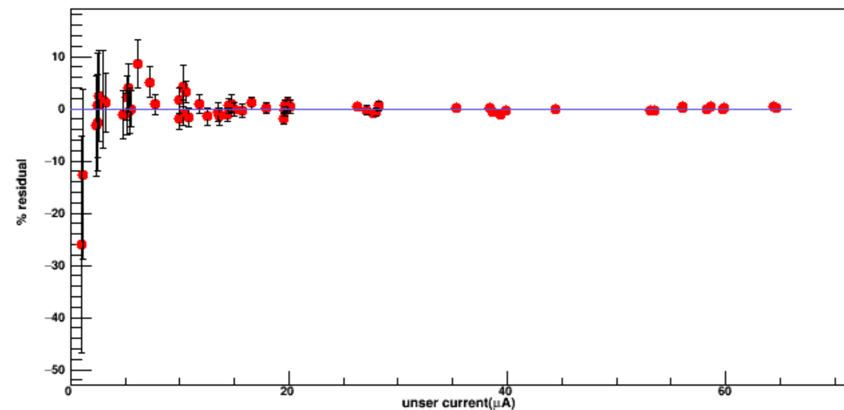
% Residual vs Unser Current
