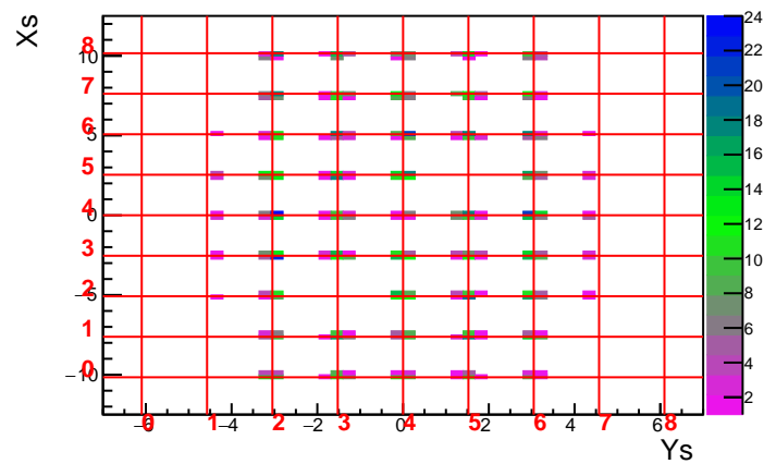
MC Run 3593 Foil 0.0 DelCut -7.5
