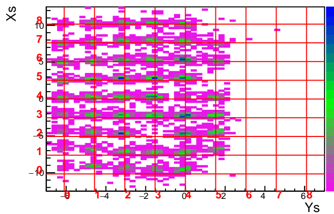
Run 3593 Foil -20.0 DelCut 7.5
