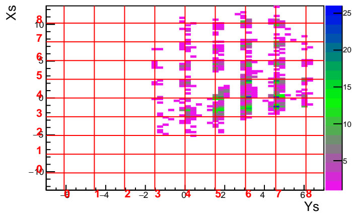
Run 3593 Foil 20.0 DelCut -7.5
