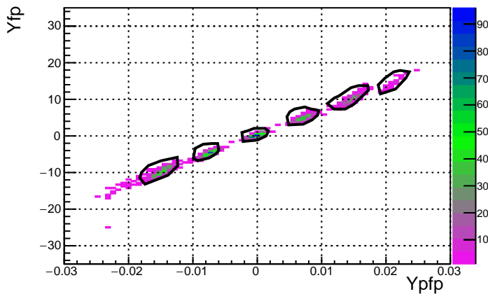
Run 3593 Foil 0.0 DelCut -6.0
