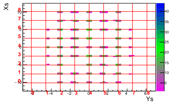
MC Run 3593 Foil 0.0 DelCut -6.0
