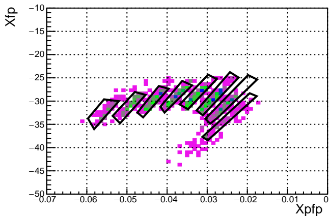
Run 3593 Foil 20.0 DelCut -7.5
