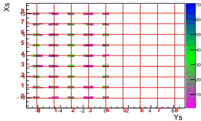
MC Run 3593 Foil -30.0 DelCut 2.5
