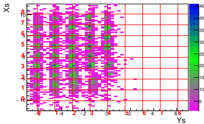
Run 3593 Foil -30.0 DelCut -2.5
