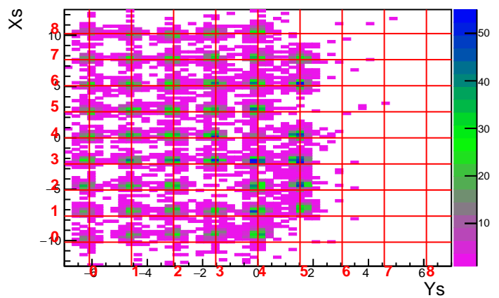
Run 3593 Foil -20.0 DelCut 2.5
