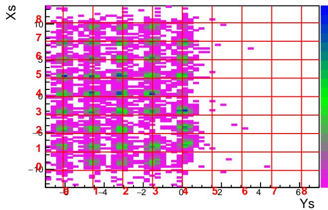
Run 3593 Foil -30.0 DelCut 2.5
