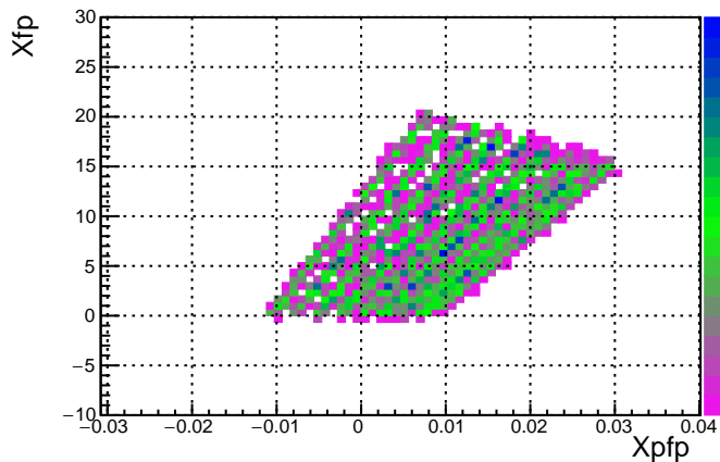
MC Run 3593 Foil -30.0 DelCut 2.5
