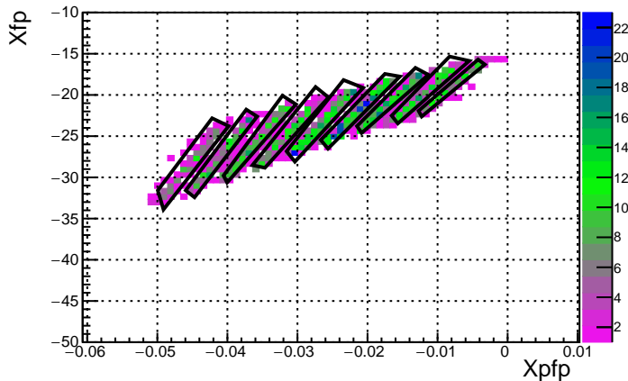
Run 3593 Foil 0.0 DelCut -6.0
