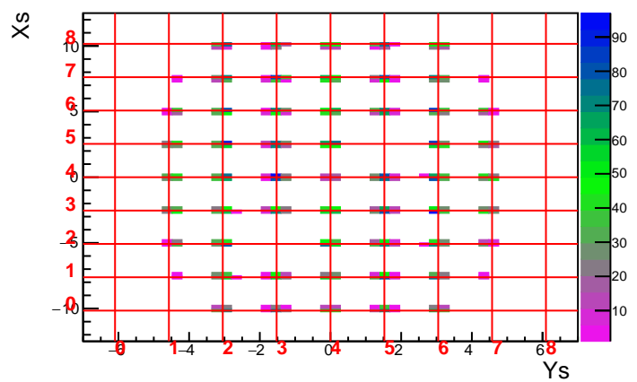
MC Run 3593 Foil 0.0 DelCut 2.5
