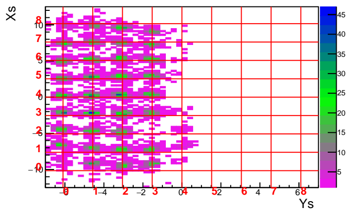
Run 3593 Foil -30.0 DelCut 7.5
