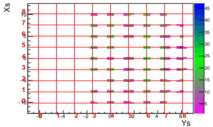
MC Run 3593 Foil 13.3 DelCut -6.0
