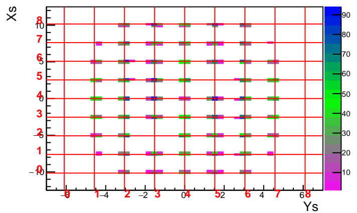
MC Run 3593 Foil 0.0 DelCut 7.5
