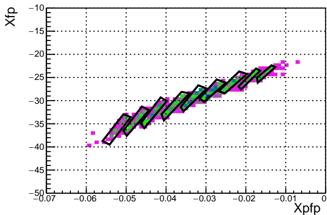
Run 3593 Foil 0.0 DelCut -7.5
