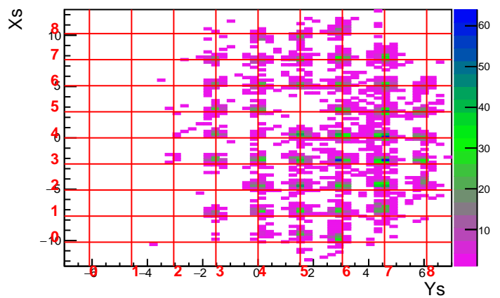
Run 3593 Foil 13.3 DelCut -2.5
