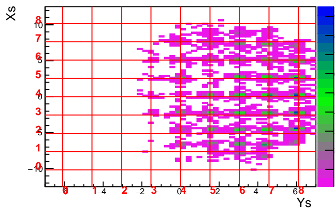
Run 3593 Foil 20.0 DelCut 2.5
