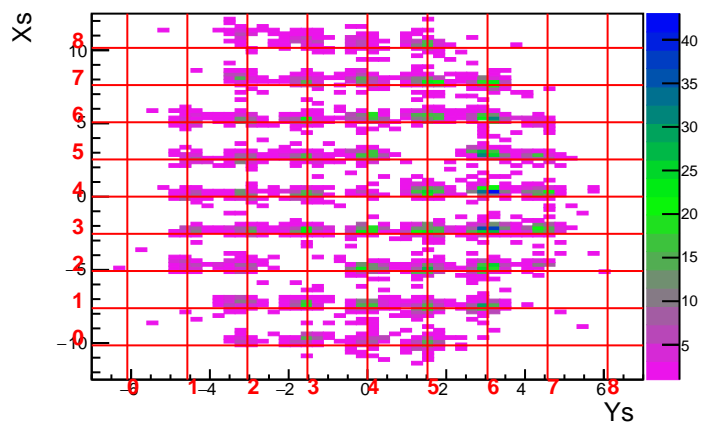
Run 3593 Foil 0.0 DelCut 7.5
