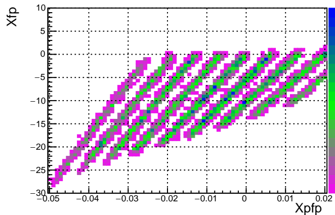
MC Run 3593 Foil 20.0 DelCut -2.5
