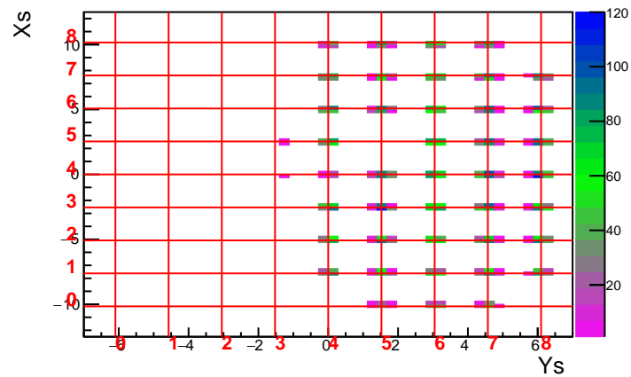
MC Run 3593 Foil 20.0 DelCut 2.5
