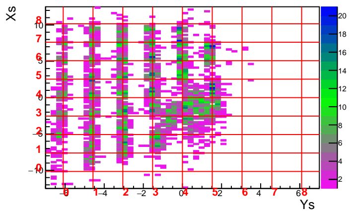
Run 3593 Foil -20.0 DelCut -6.0
