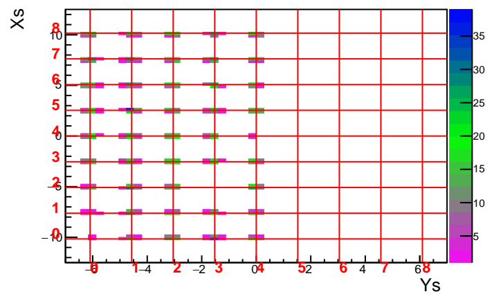
MC Run 3593 Foil -30.0 DelCut -6.0
