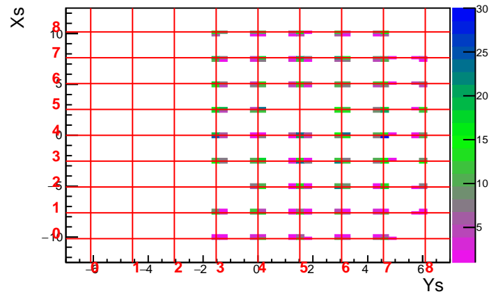
MC Run 3593 Foil 13.3 DelCut -7.5
