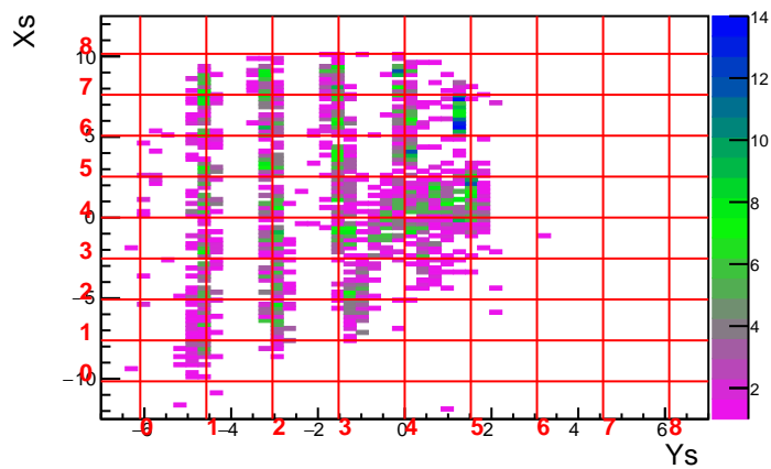
Run 3593 Foil -20.0 DelCut -7.5
