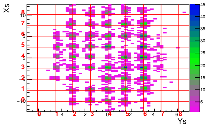
Run 3593 Foil 0.0 DelCut -2.5
