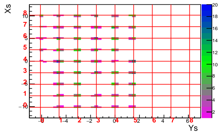
MC Run 3593 Foil -20.0 DelCut -7.5
