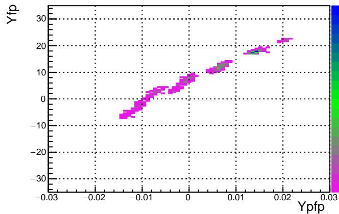
MC Run 3593 Foil -30.0 DelCut -7.5
