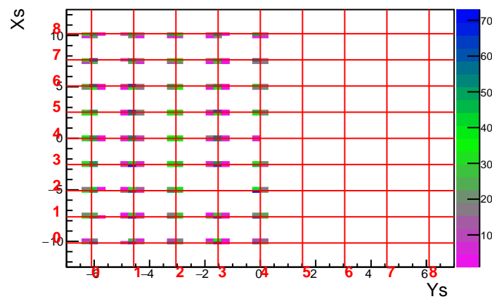
MC Run 3593 Foil -30.0 DelCut -2.5
