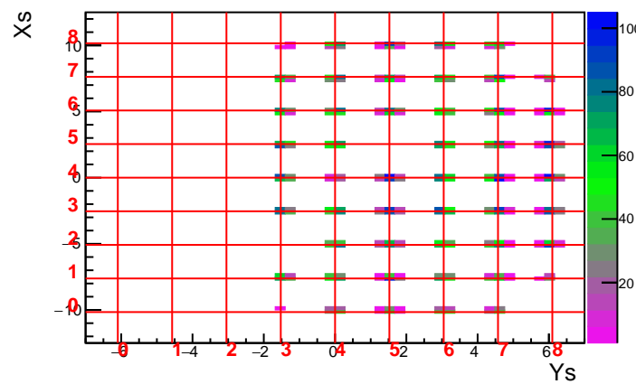
MC Run 3593 Foil 13.3 DelCut 2.5
