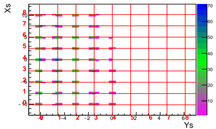
MC Run 3593 Foil -30.0 DelCut 7.5
