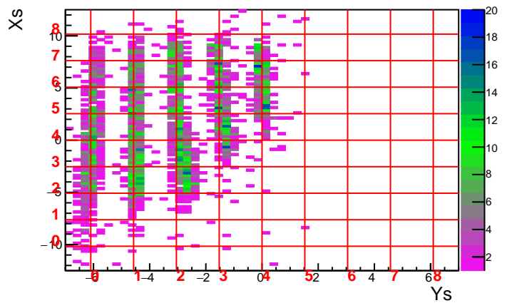
Run 3593 Foil -30.0 DelCut -6.0
