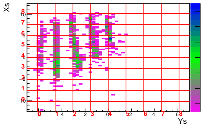
Run 3593 Foil -30.0 DelCut -7.5
