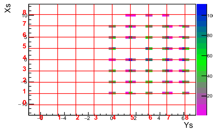
MC Run 3593 Foil 20.0 DelCut 7.5
