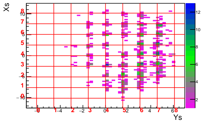
Run 3593 Foil 13.3 DelCut -7.5
