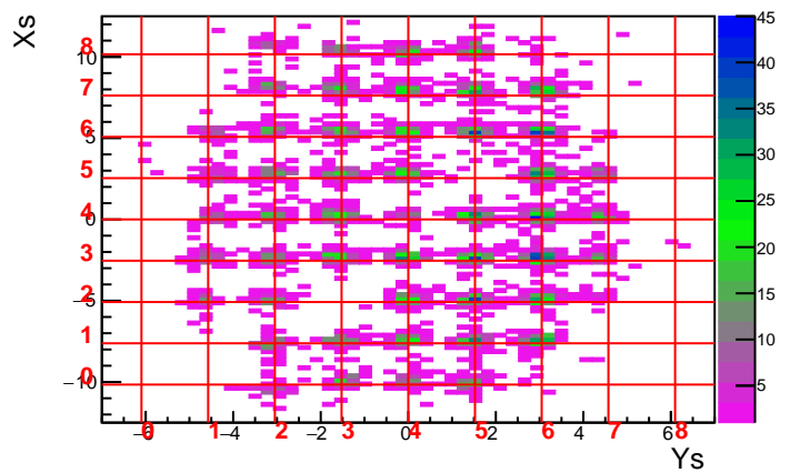
Run 3593 Foil 0.0 DelCut 2.5
