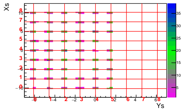
MC Run 3593 Foil -20.0 DelCut -6.0
