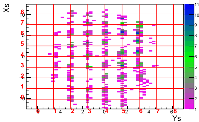
Run 3593 Foil 0.0 DelCut -7.5
