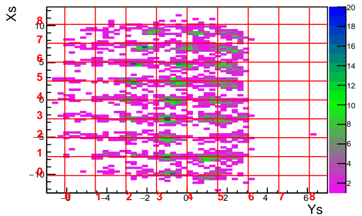
Run 3610 Foil -20.0 DelCut 7.5
