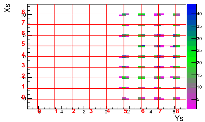
MC Run 3610 Foil 20.0 DelCut -7.0
