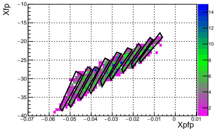
Run 3610 Foil 0.0 DelCut -7.0
