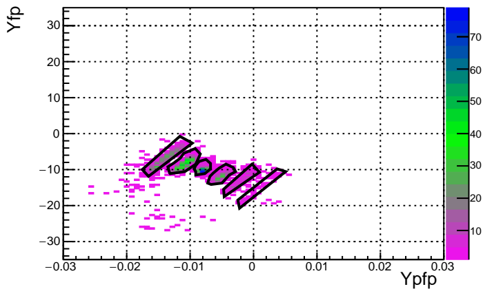
Run 3610 Foil 13.3 DelCut 2.5
