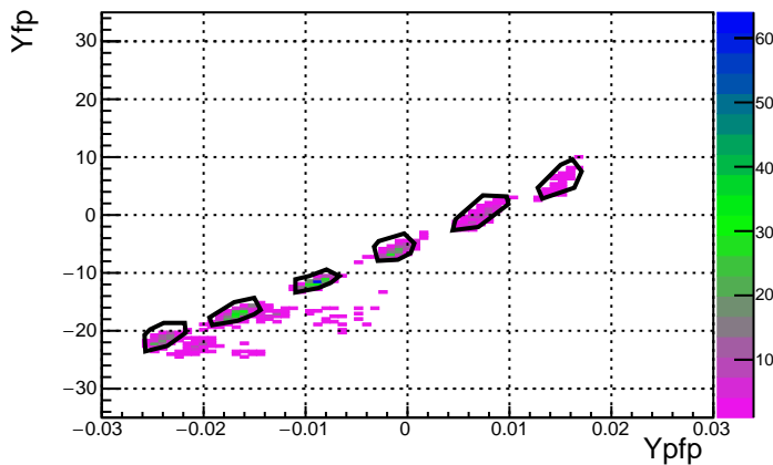
Run 3610 Foil 13.3 DelCut -7.0
