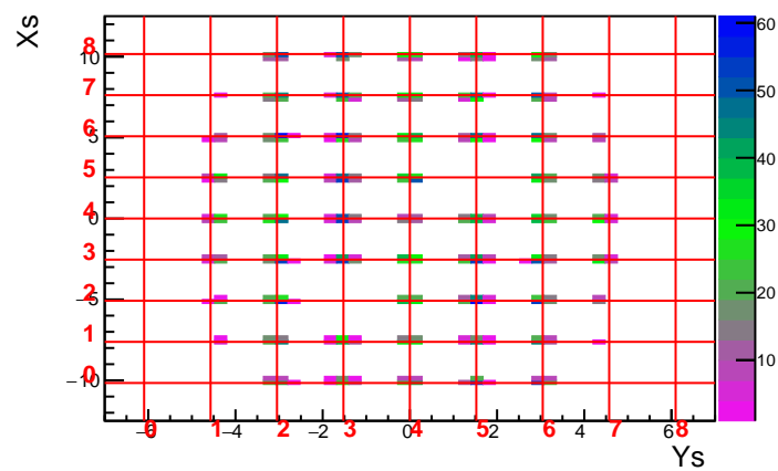
MC Run 3610 Foil 0.0 DelCut -1.5
