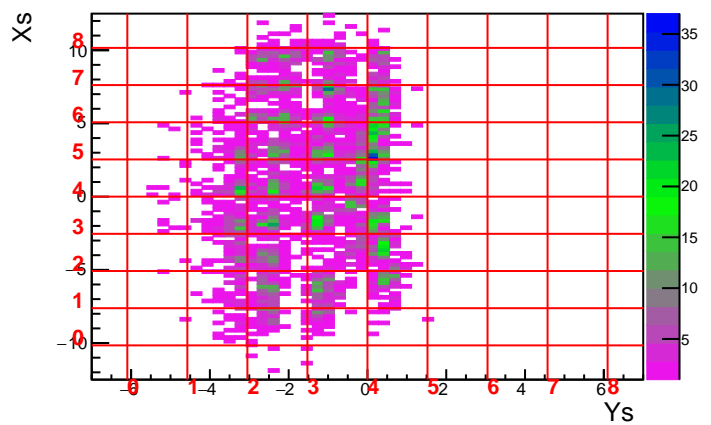
Run 3610 Foil -20.0 DelCut -4.5
