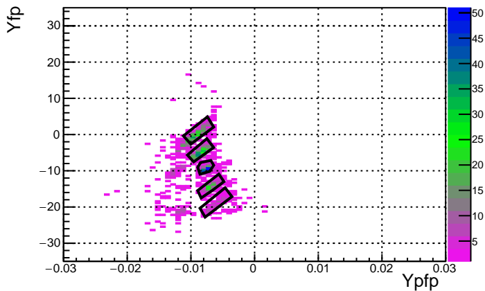
Run 3610 Foil 13.3 DelCut 7.5
