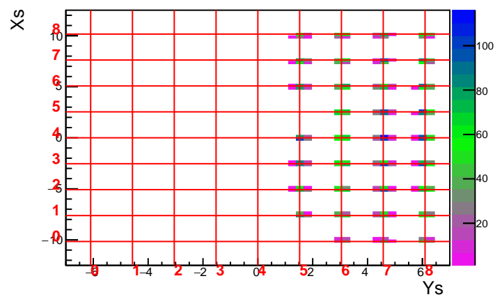
MC Run 3610 Foil 20.0 DelCut 2.5
