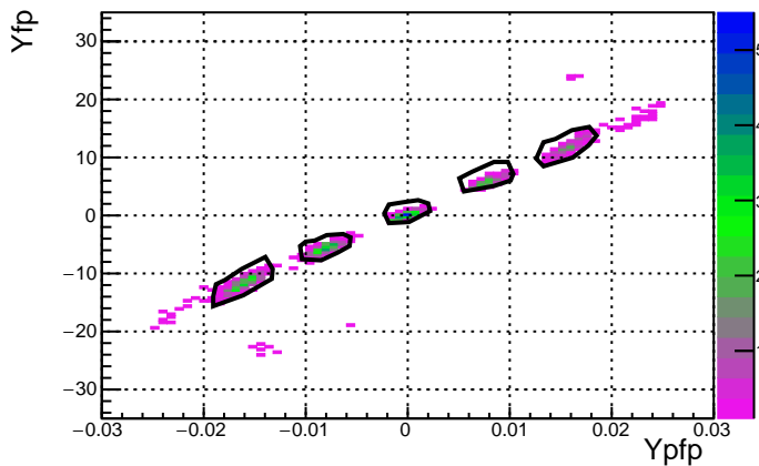
Run 3610 Foil 0.0 DelCut -7.0
