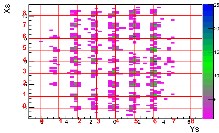
Run 3610 Foil 0.0 DelCut -4.5
