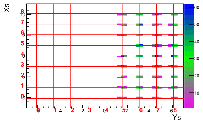
MC Run 3610 Foil 20.0 DelCut -4.5
