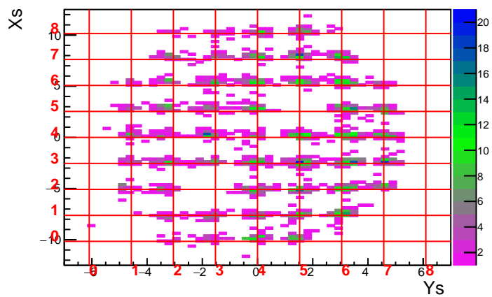
Run 3610 Foil 0.0 DelCut 7.5
