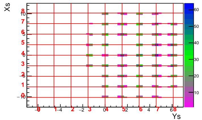
MC Run 3610 Foil 13.3 DelCut -4.5
