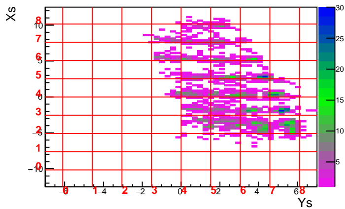
Run 3610 Foil 20.0 DelCut 2.5
