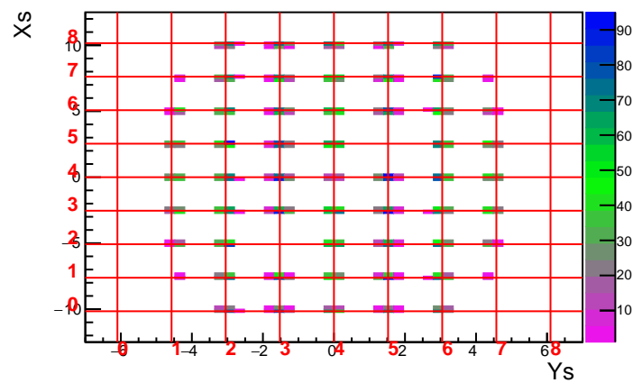
MC Run 3610 Foil 0.0 DelCut 2.5
