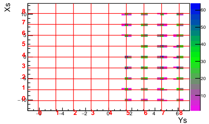
MC Run 3610 Foil 20.0 DelCut -1.5
