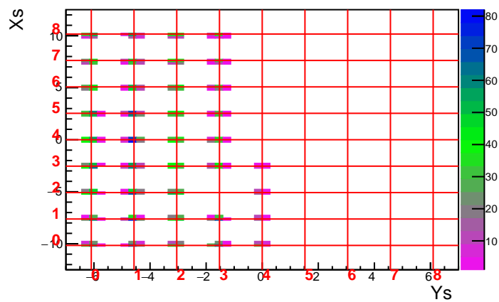
MC Run 3610 Foil -20.0 DelCut 7.5
