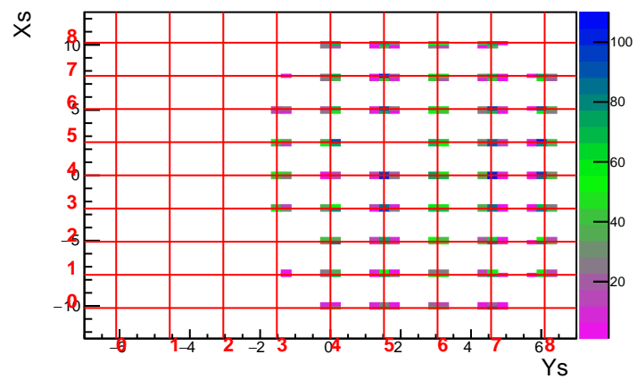
MC Run 3610 Foil 13.3 DelCut 2.5
