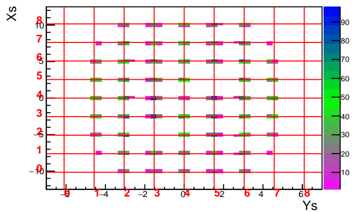
MC Run 3610 Foil 0.0 DelCut 7.5
