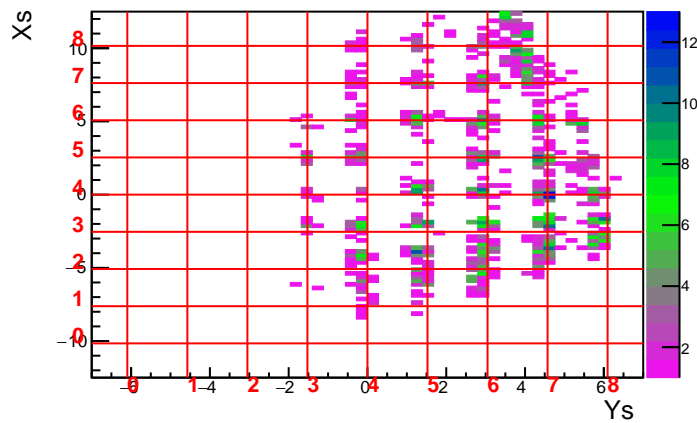
Run 3610 Foil 13.3 DelCut -7.0
