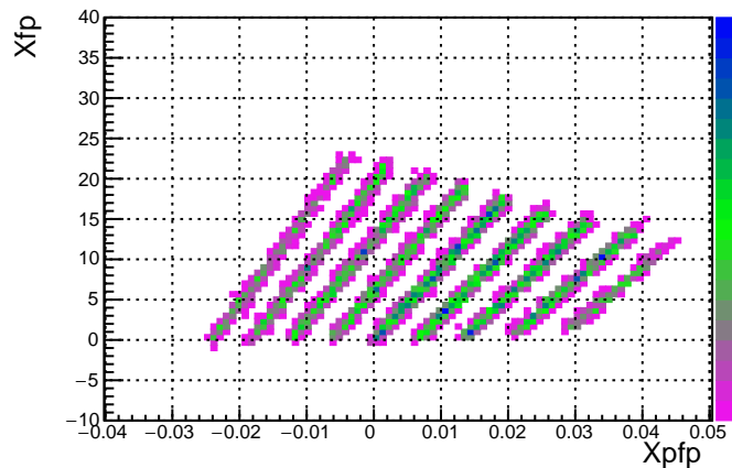
MC Run 3610 Foil 20.0 DelCut 2.5
