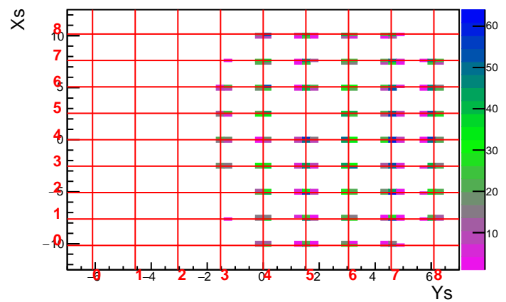
MC Run 3610 Foil 13.3 DelCut -1.5
