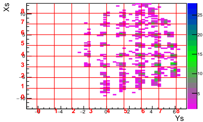
Run 3610 Foil 13.3 DelCut -4.5
