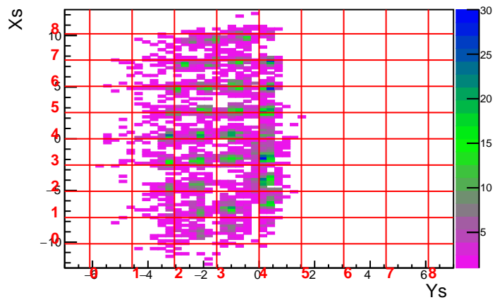
Run 3610 Foil -20.0 DelCut -1.5
