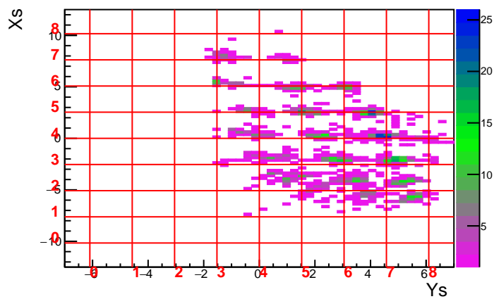
Run 3610 Foil 20.0 DelCut 7.5
