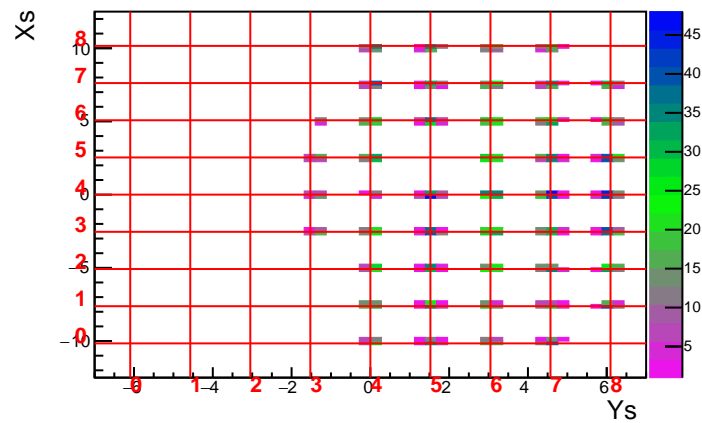
MC Run 3610 Foil 13.3 DelCut -7.0
