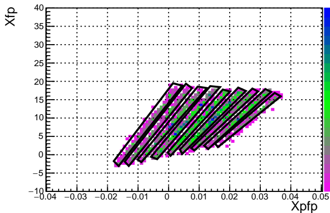
Run 3610 Foil -20.0 DelCut 2.5
