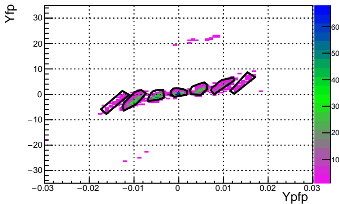
Run 3610 Foil 0.0 DelCut -1.5
