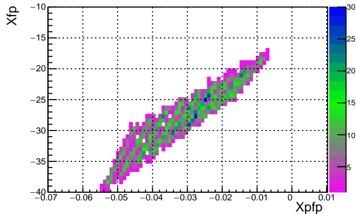
MC Run 3610 Foil 0.0 DelCut -7.0
