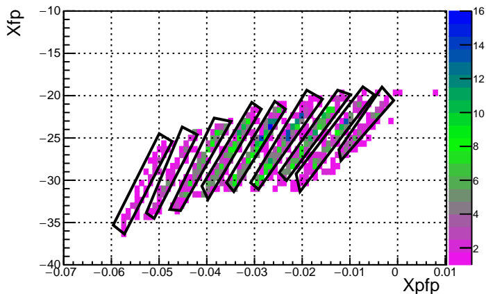
Run 3610 Foil 20.0 DelCut -7.0
