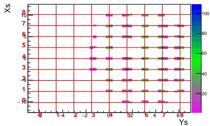
MC Run 3610 Foil 13.3 DelCut 7.5
