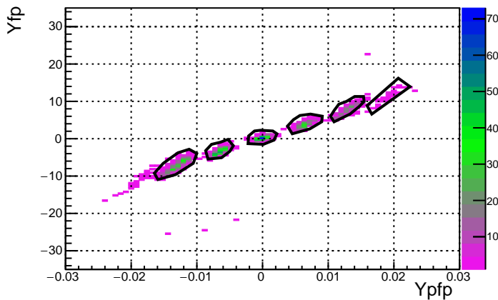
Run 3610 Foil 0.0 DelCut -4.5
