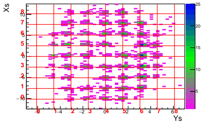
Run 3610 Foil 0.0 DelCut 2.5
