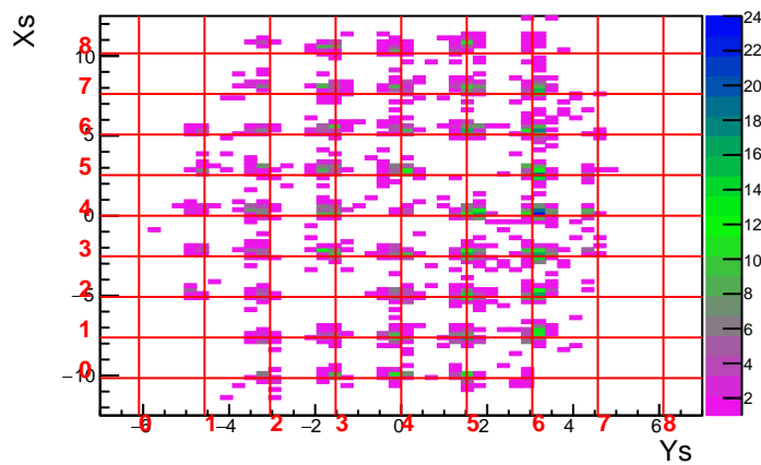
Run 3610 Foil 0.0 DelCut -1.5
