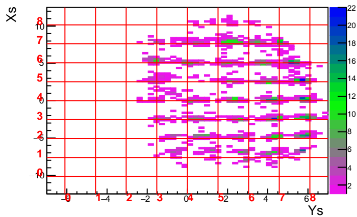
Run 3610 Foil 13.3 DelCut 7.5
