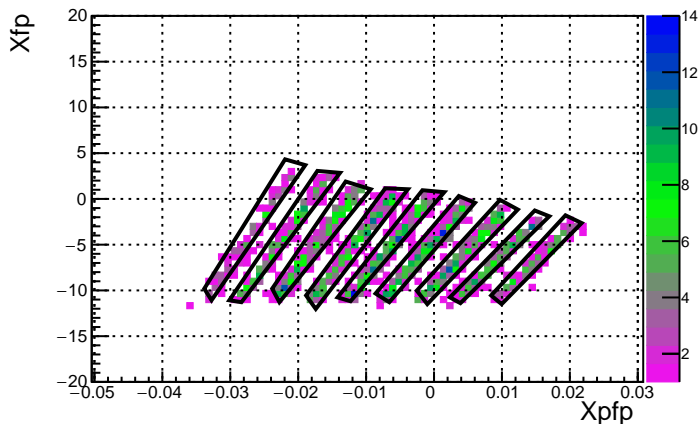
Run 3610 Foil 13.3 DelCut -1.5
