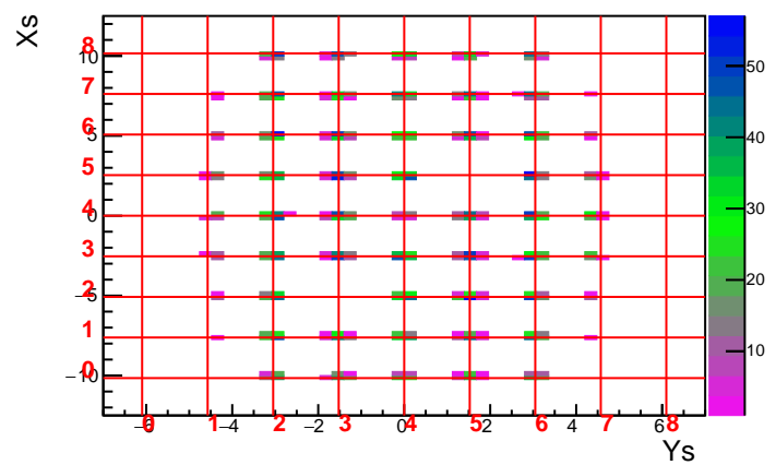
MC Run 3610 Foil 0.0 DelCut -4.5
