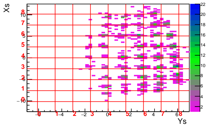
Run 3610 Foil 13.3 DelCut -1.5
