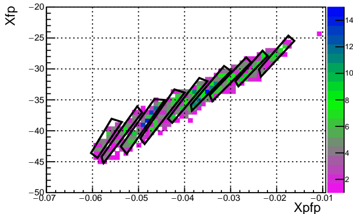
Run 3610 Foil 0.0 DelCut -9.0
