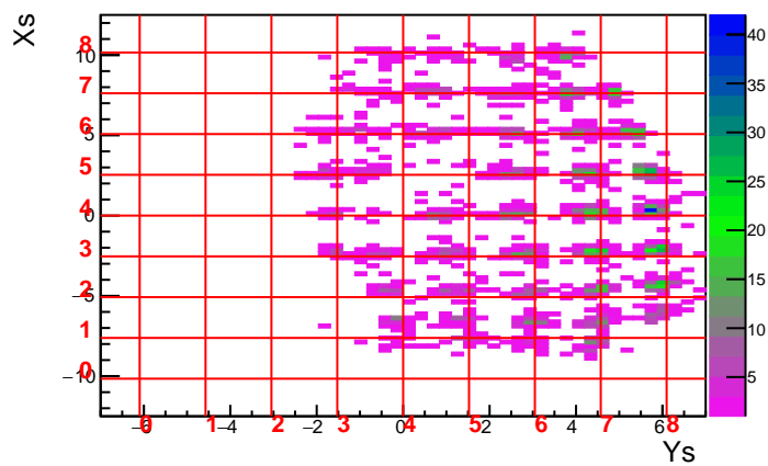
Run 3610 Foil 13.3 DelCut 2.5
