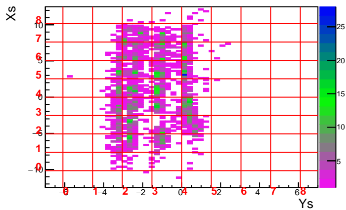
Run 3610 Foil -20.0 DelCut -7.0
