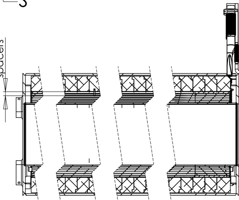
COUPE U-U
