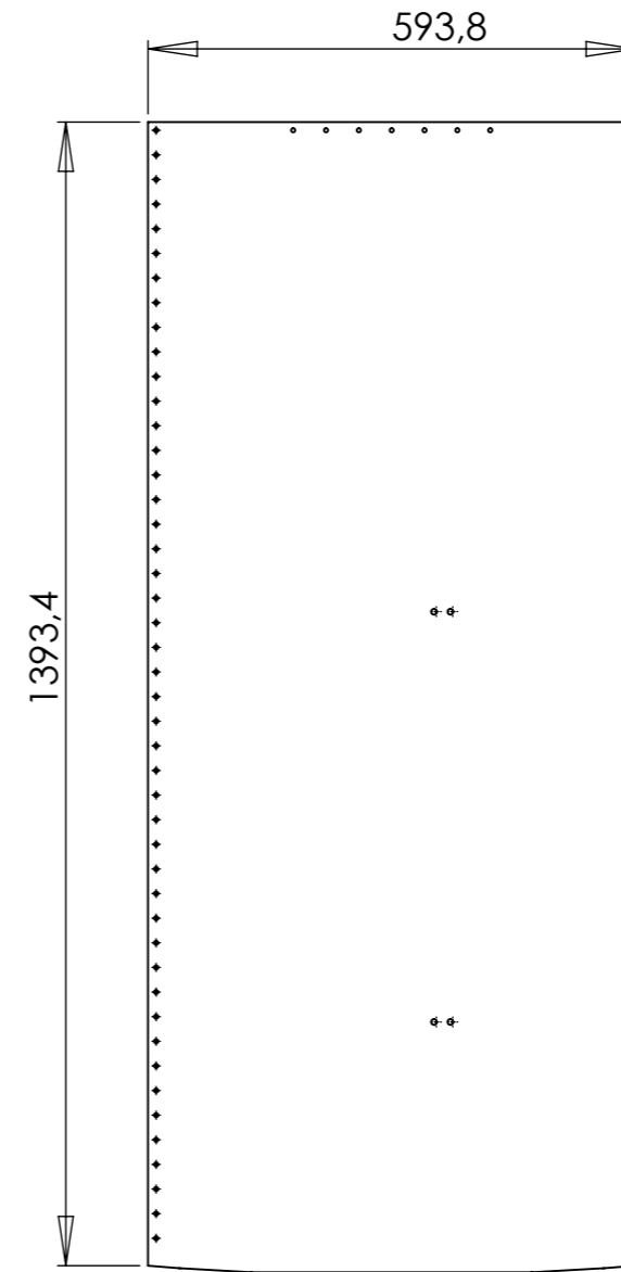
FLAT PATTERN
