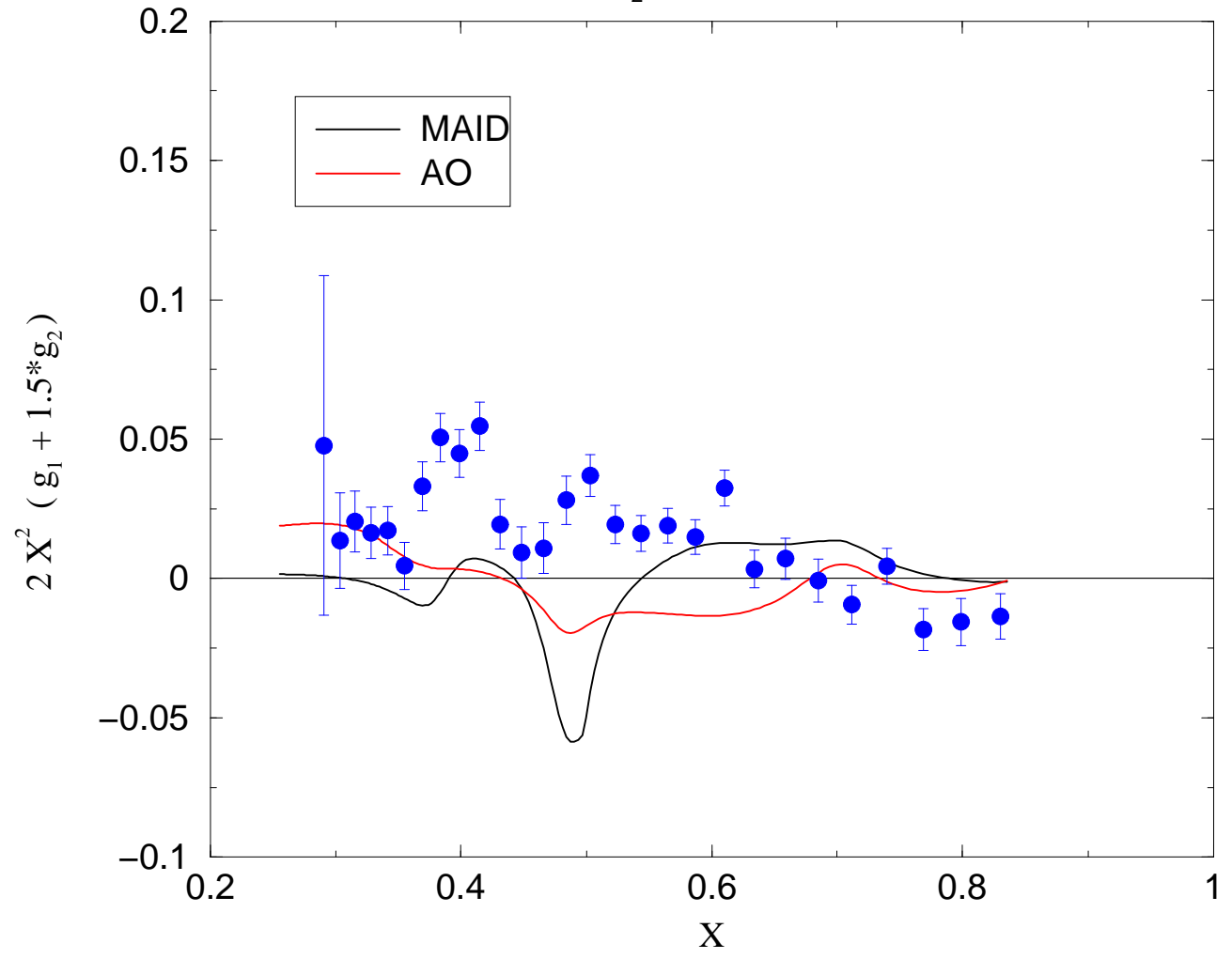
d_2 Integrand
