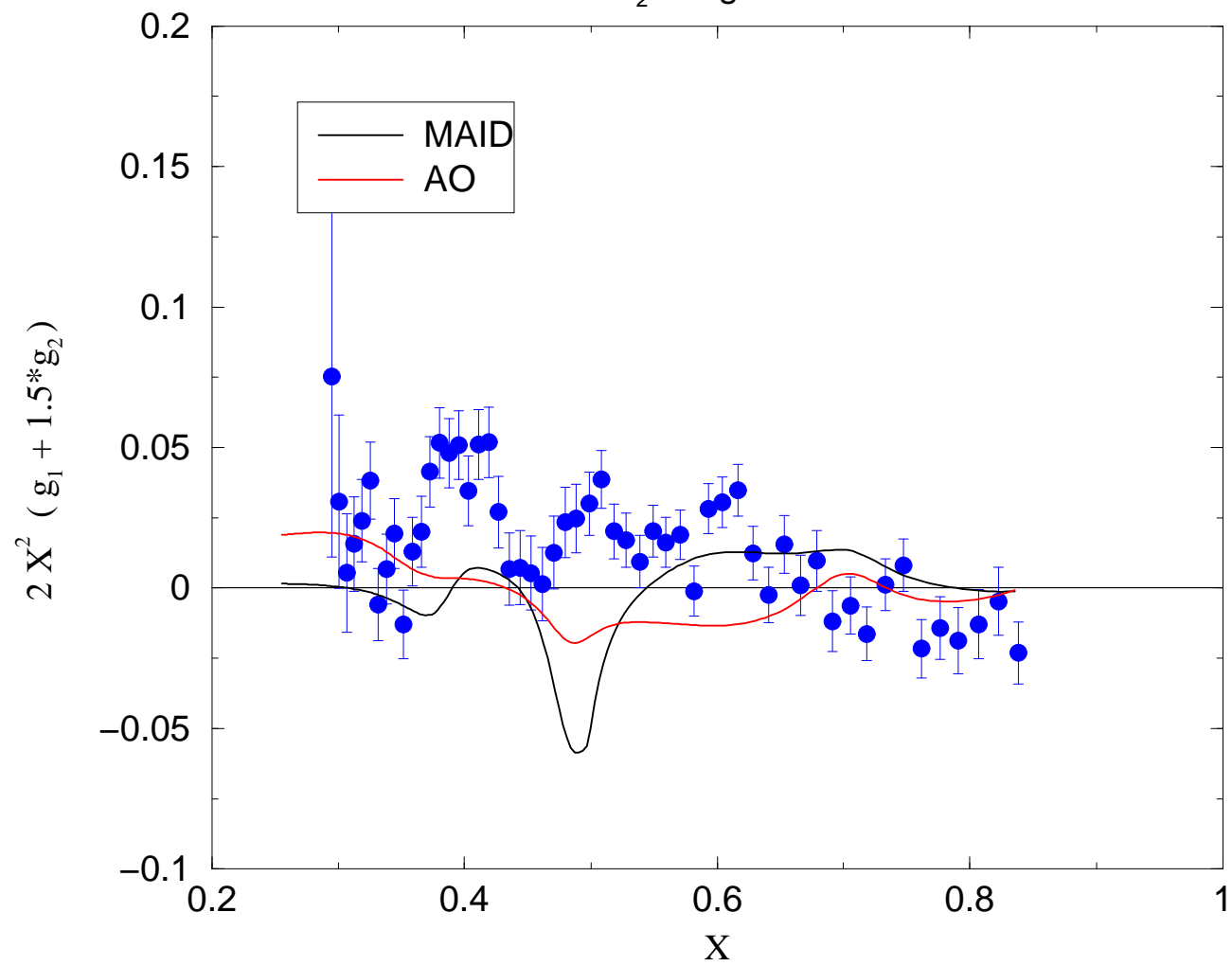
d_2 Integrand
