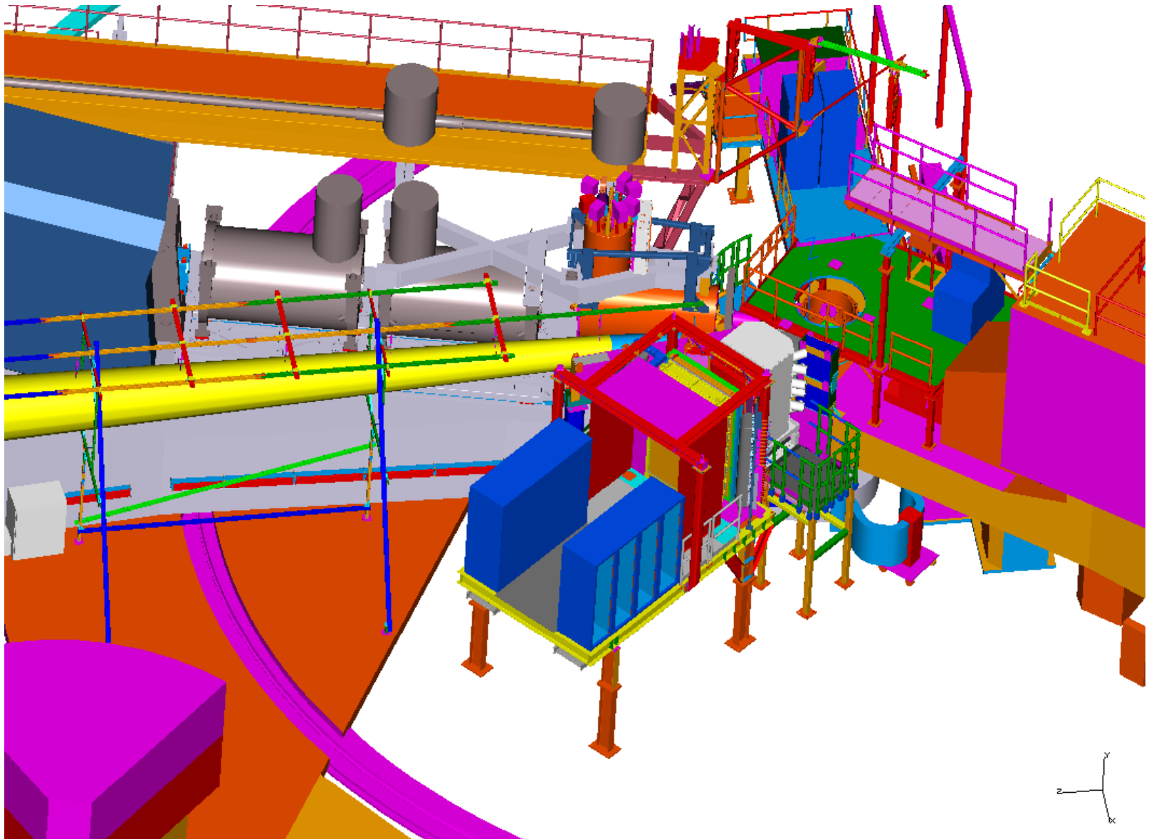
SANE LAYOUT Shielding and Supports
