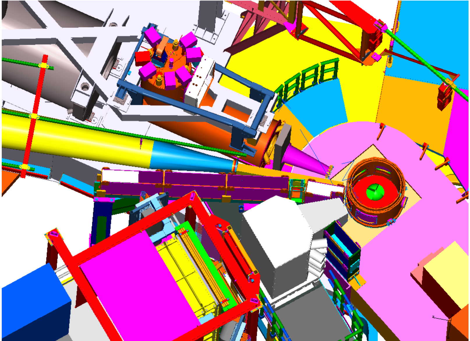
View of Beamline shielding-Polarized Target Platform removed
