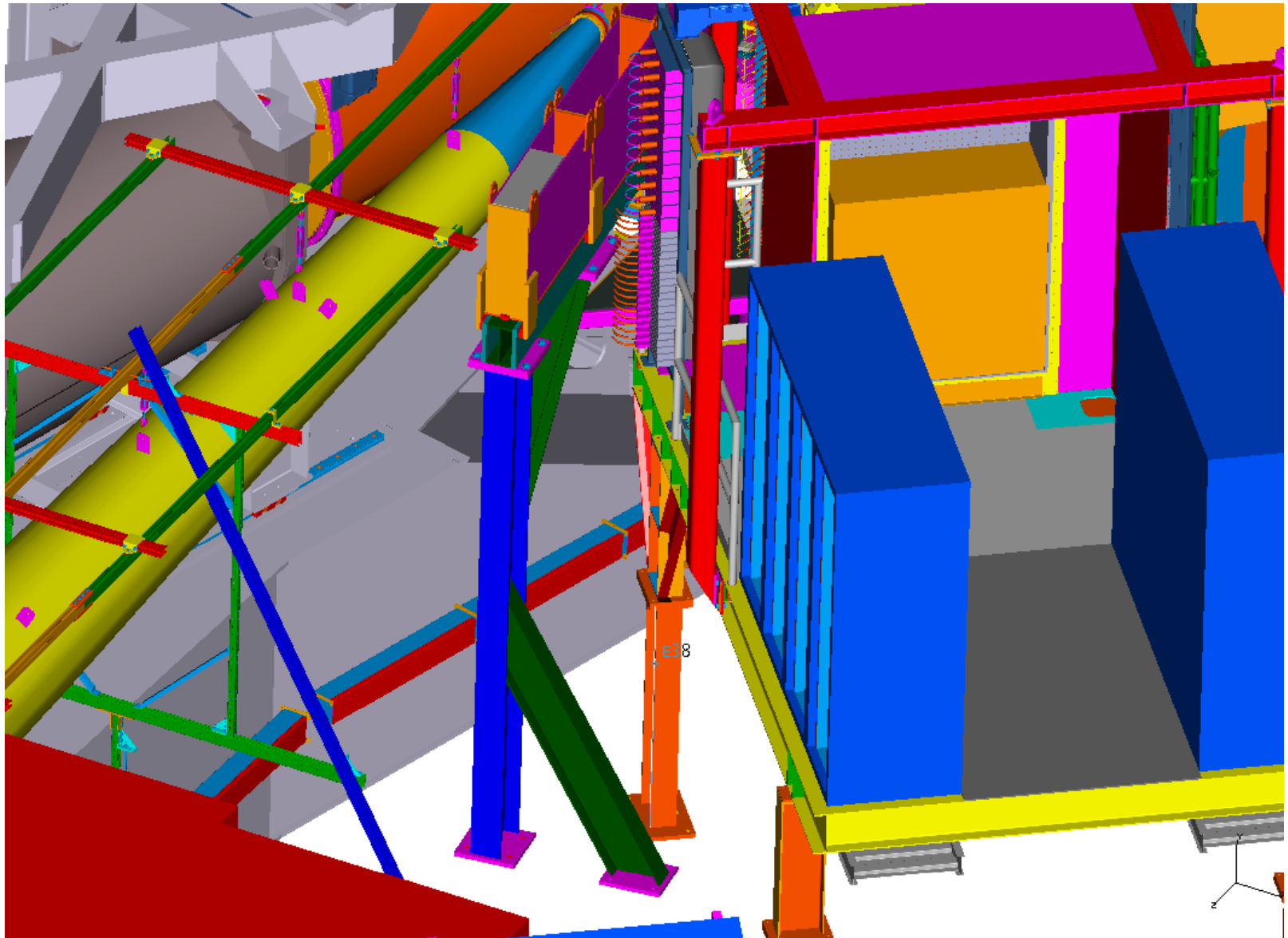
Shielding Support, Beamline
