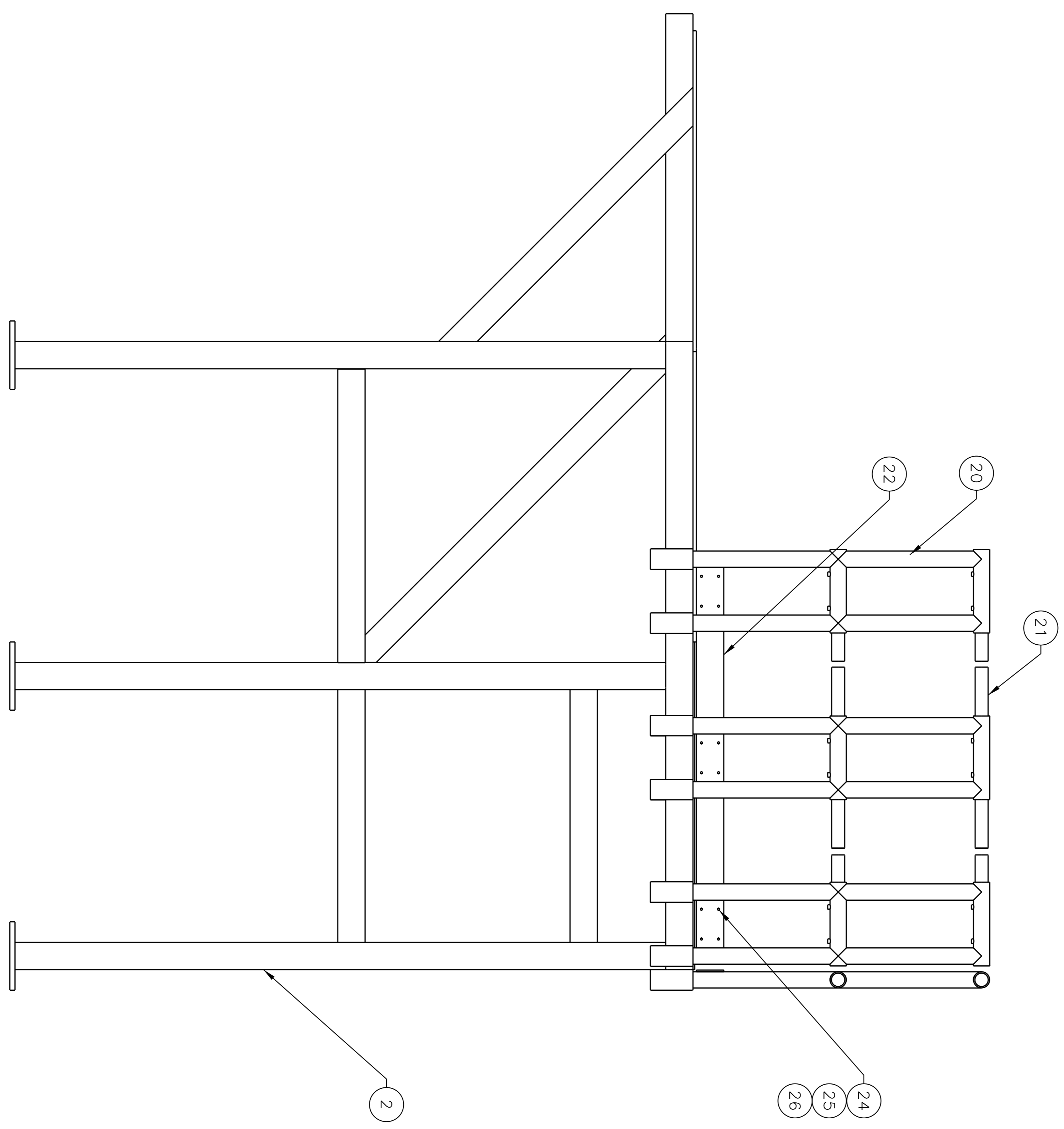
-01 SANE CHERENKOV SUPPORT STAND ASSY SCALE 1/10
