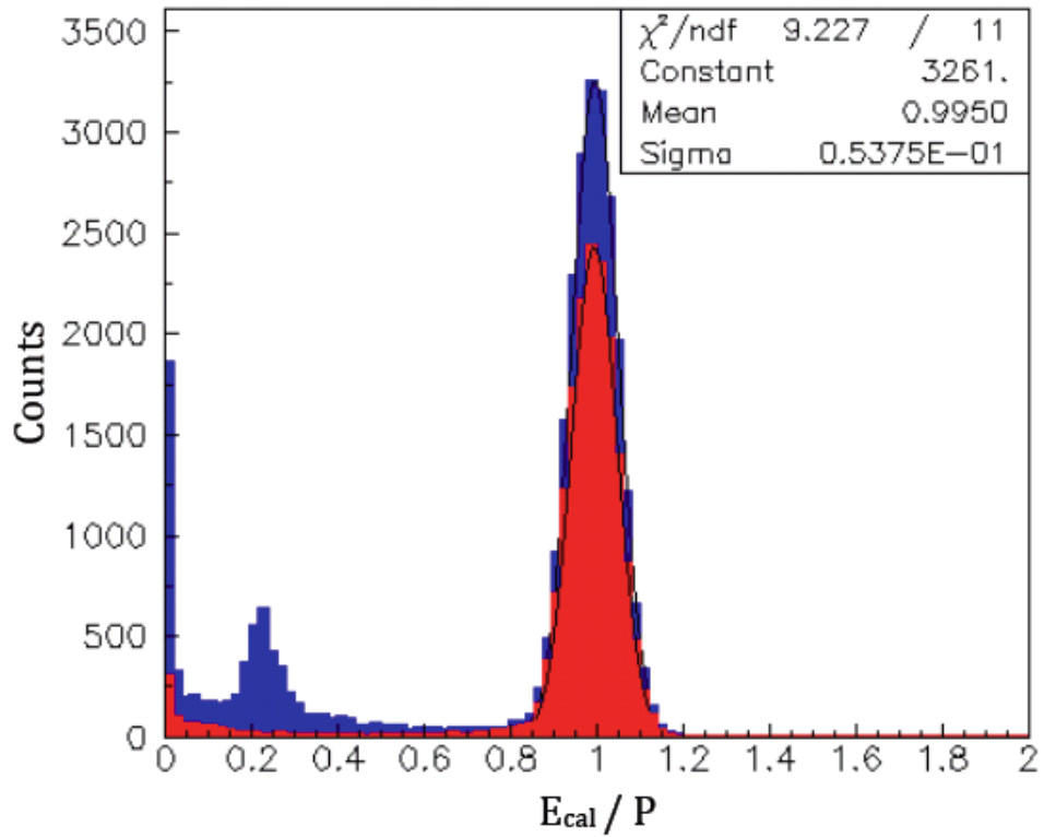
Figure 3.2: The ratio of calorimeter deposited energy E_{cal} to momentum P (Blue), showing electron peak at E_{cal}/P 1. After applying Čerenkov photoelectron cut (Red), pion signal is greatly reduced [19].
