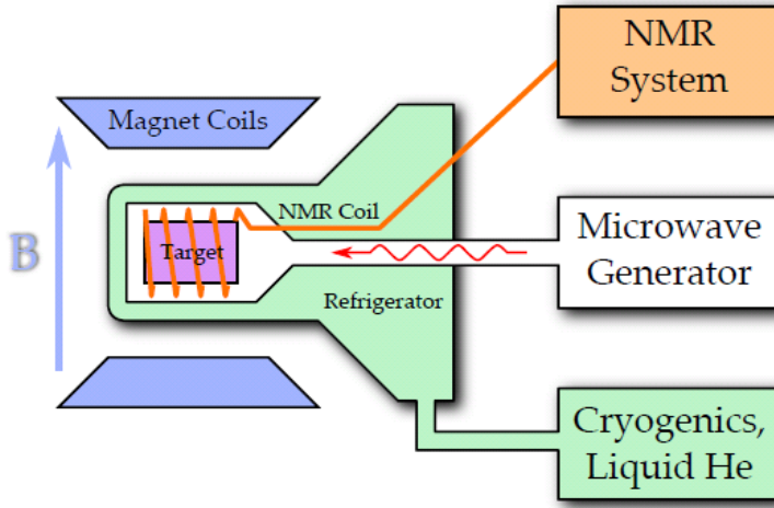
Figure 2.9: Schematics of the target system: cryogenic, magnetic field, microwave, NMR
