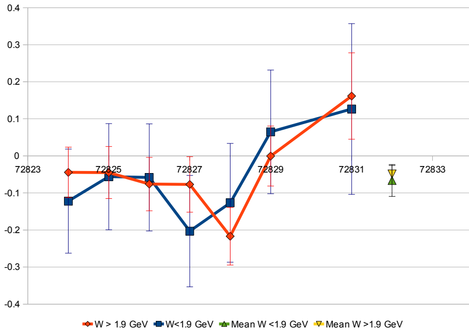
Asymmetry for 4.7 GeV 80° runs
