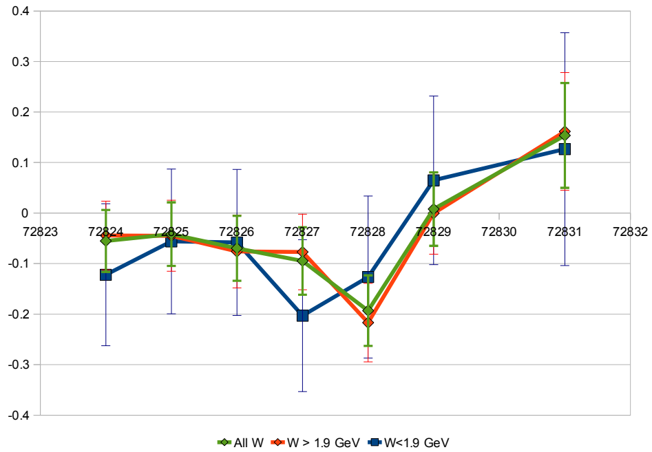
Asymmetry for 4.7 GeV 80° runs
