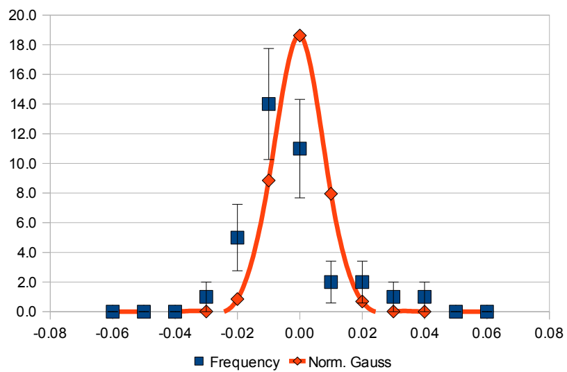
Histogram of A_{\text{raw\_perp}} and Gaussian with mean = \langle A \rangle , width = \sigma_A
