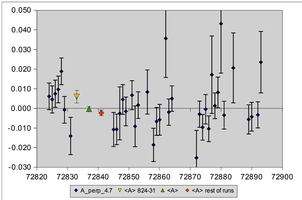
A_{\text{perp}_4.7_{\text{raw}}} by run number.
