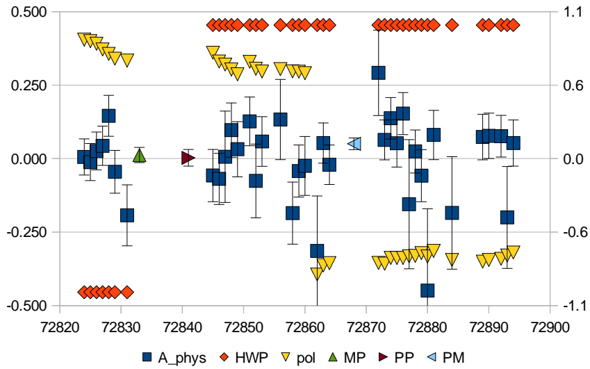
A_phys 4.7 80° all runs using trig+/- and scaler 513/514
