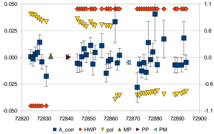
A_perp_4.7 all runs using trig+/- and scaler 513/514
