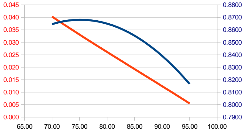
5.9 GeV 50° W=2
