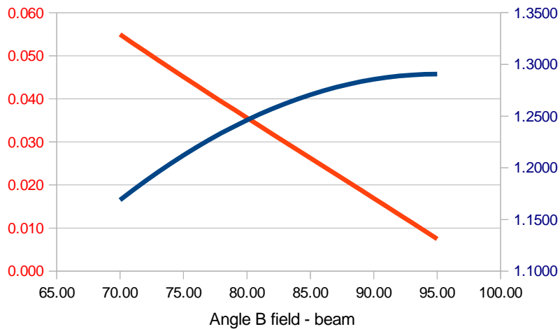
4.7 GeV 30° W=2
