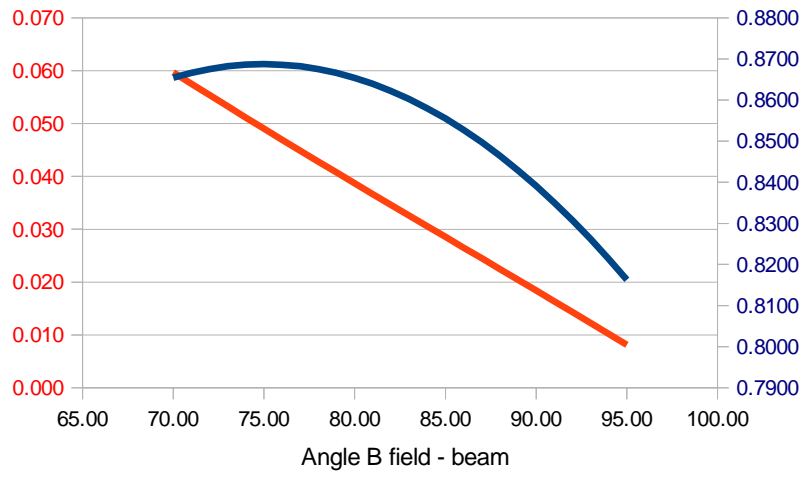
4.7 GeV 50° W=2
