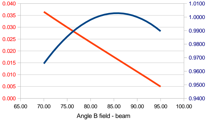
5.9 GeV 40° W=2
