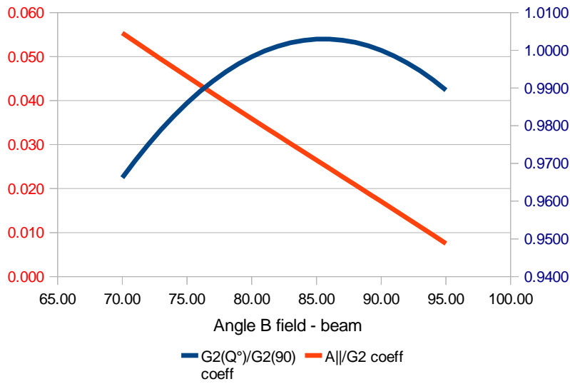
4.7 GeV 40° W=2
