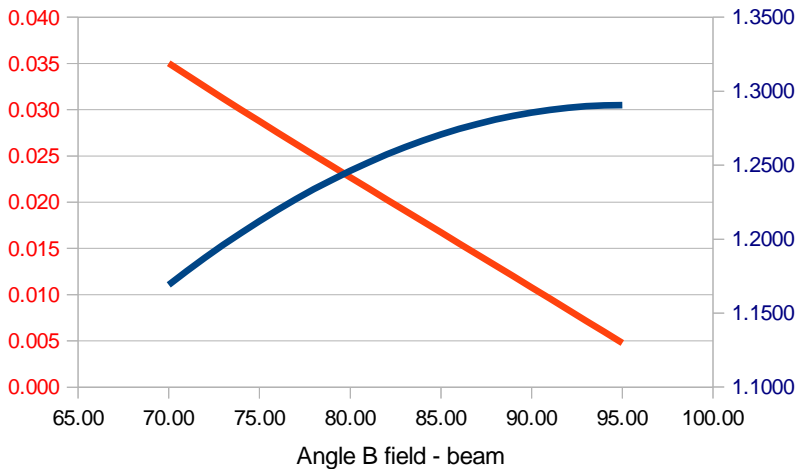
5.9 GeV 30° W=2
