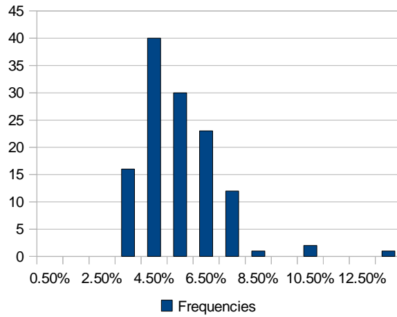
cerh=0, E<1.3 GeV (was 0.8)
