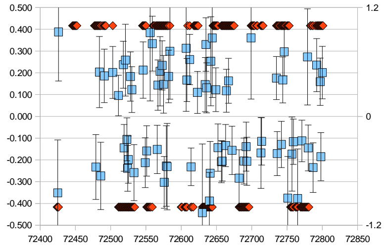
cer_h > 0 E > .8
