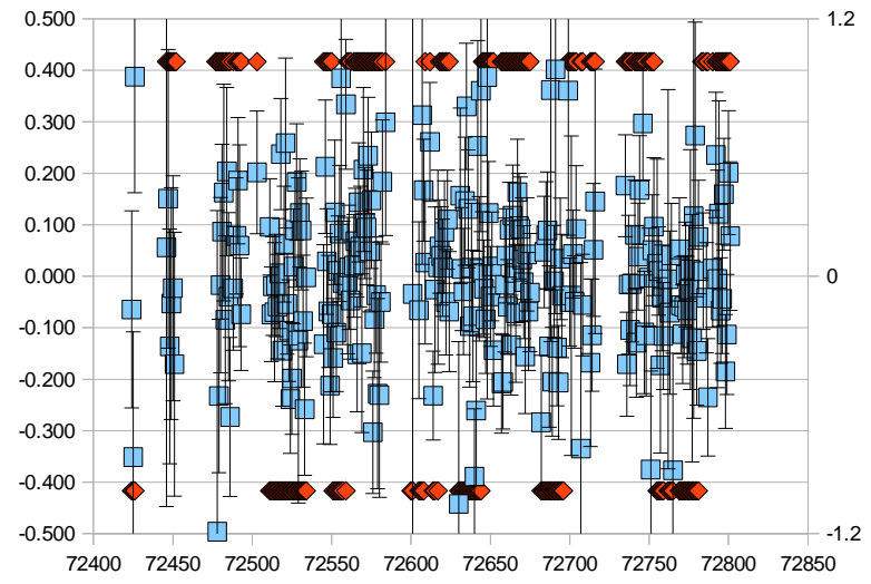
cer_h > 0 E > .8
