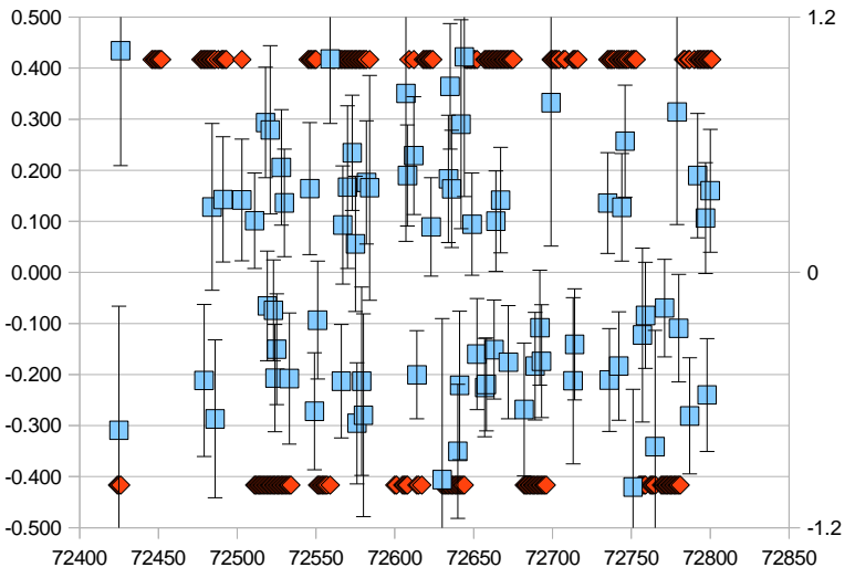
cer_h > 0 E > .8
