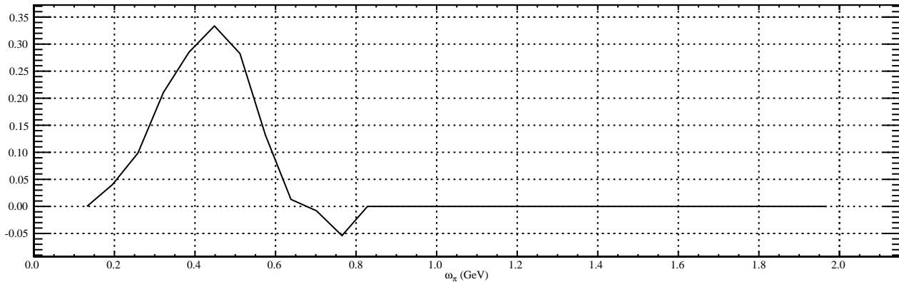
\pi^0 Asymmetry
