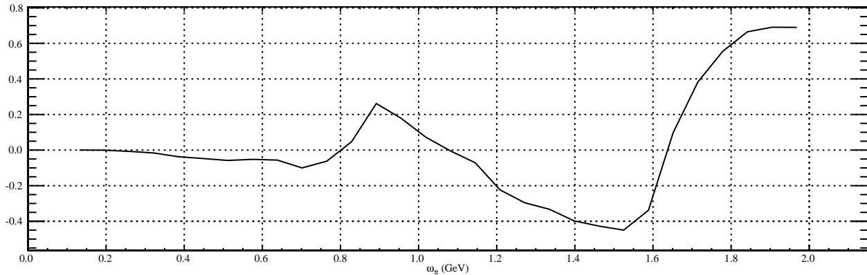
\pi^0 Asymmetry
