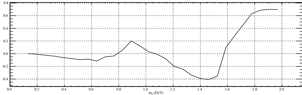
\pi^0 Asymmetry
