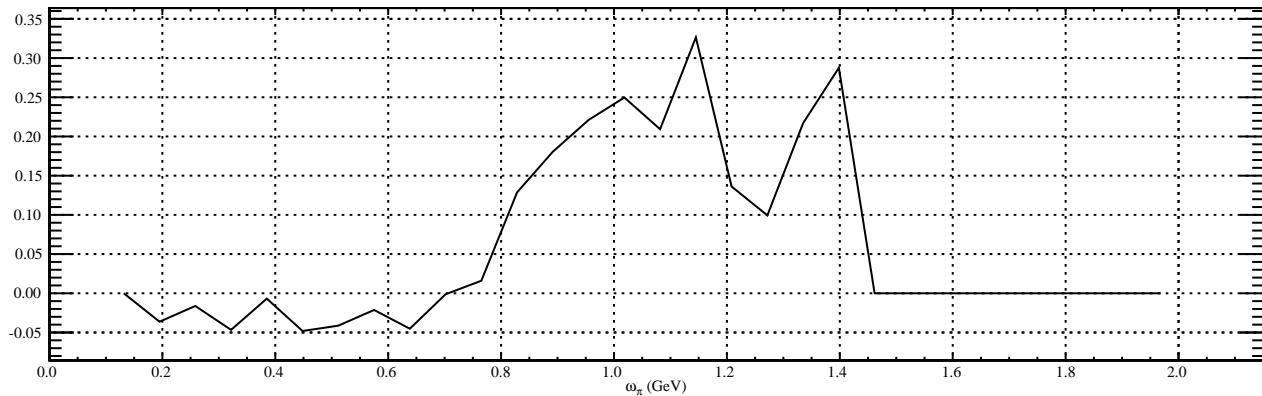
\pi^0 Asymmetry
