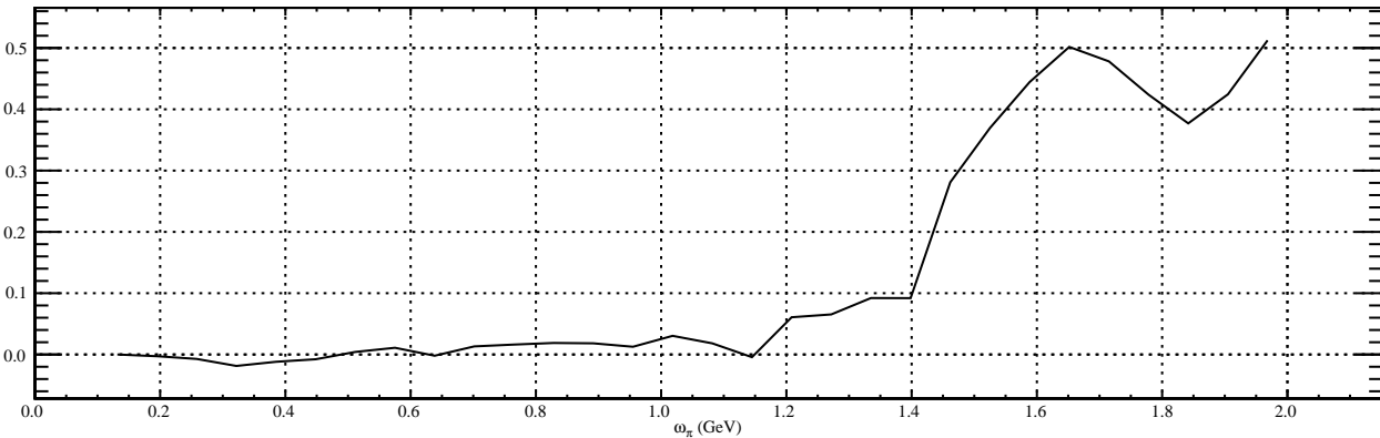
\pi^0 Asymmetry
