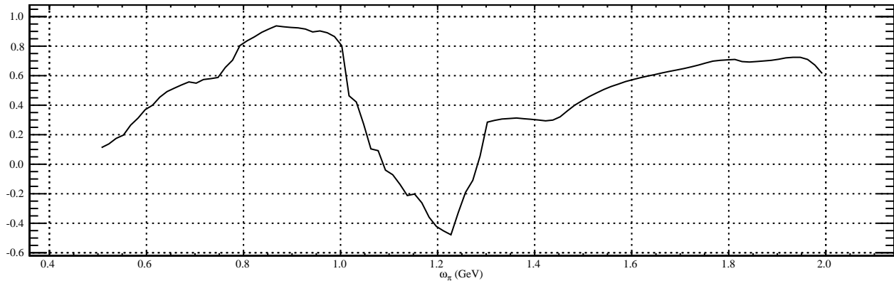
\pi^0 Asymmetry
