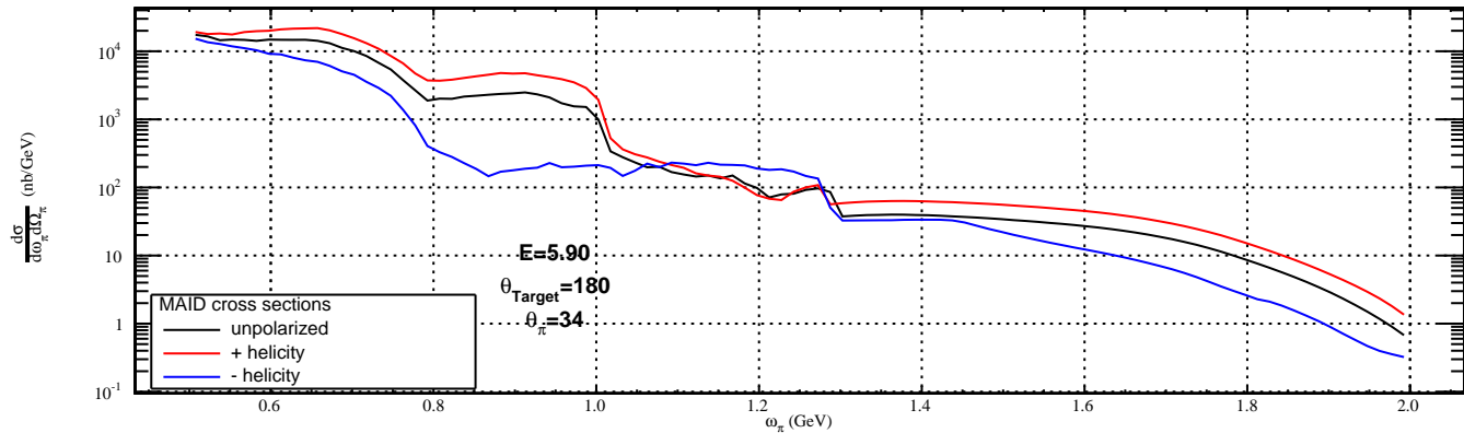
\pi^0 Asymmetry
