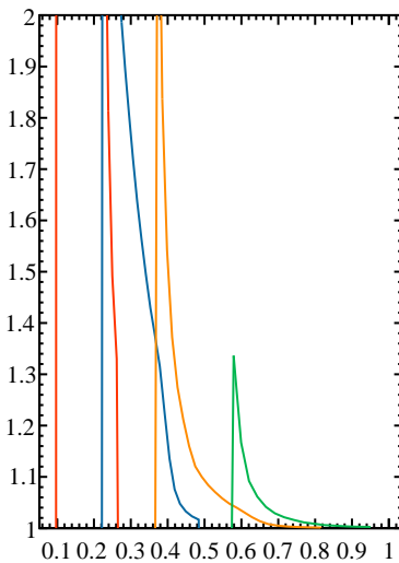
1/f_{bg}
