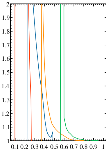
C_{bg}
