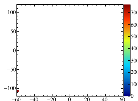
bigalClusters.fVMoment:bigalClusters.fVMoment (fThrownParticles.fPdgCode==11)
