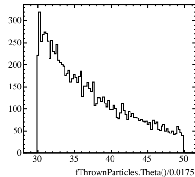
fThrownParticles.Theta()/0.0175 (fThrownParticles.fPdgCode==11)
