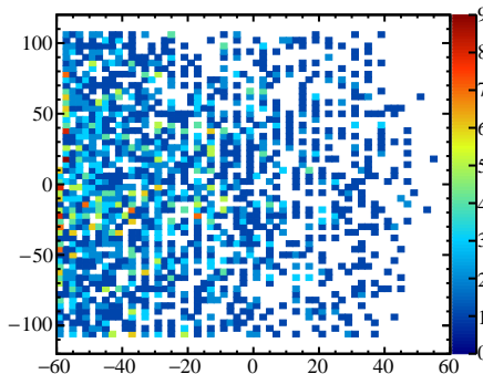
bigalClusters.fVMoment:bigalClusters.fVMoment (fThrownParticles.fPdgCode==11)
