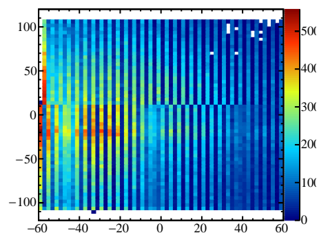
bigalClusters.fVMoment:bigalClusters.fVMoment (fThrownParticles.fPdgCode==11)
