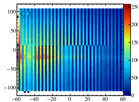
bigalClusters.fVMoment:bigalClusters.fNMoment (fThrownParticles.fPdgCode==11)
