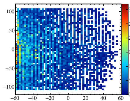
bigalClusters.fVMoment:bigalClusters.fNMoment (fThrownParticles.fPdgCode==11)
