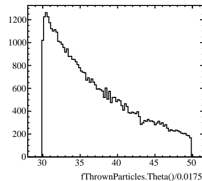
fThrownParticles.Theta()/0.0175 (fThrownParticles.fPdgCode==11)
