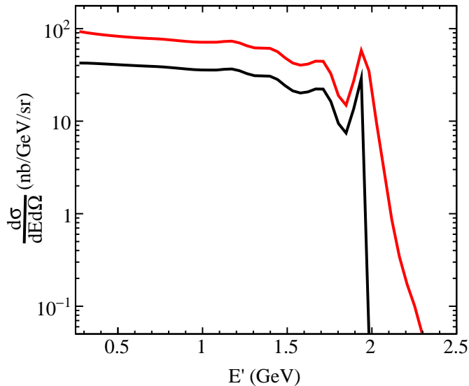
F1F209 born DIS cross-section
