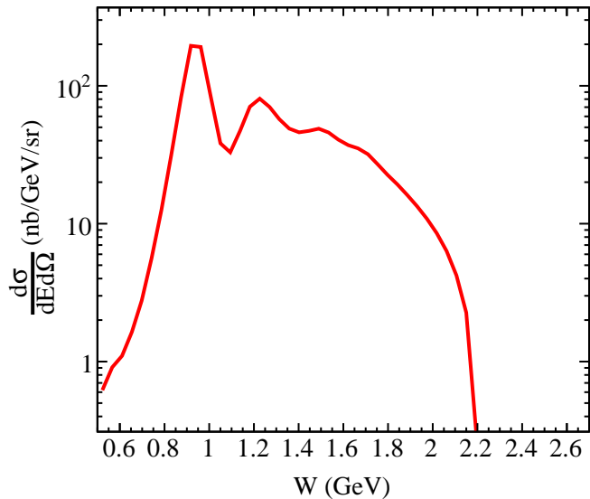
F1F209 born DIS cross-section
