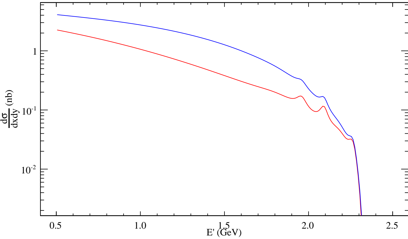
POLRAD Born cross-section
