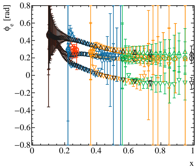
\phi vs x
