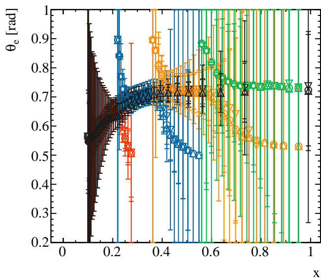
\theta vs x
