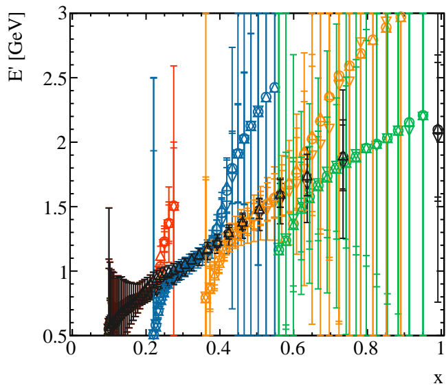
E' vs x
