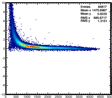
fDelta_Theta*180.0/TMath::Pi():fClusterEnergy
