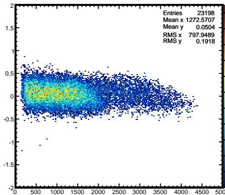
fDelta_Theta*180.0/TMath::Pi():fClusterEnergy
