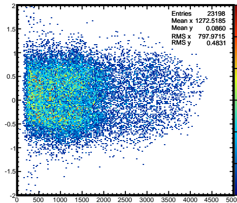
fDelta_Phi*180.0/TMath::Pi():fClusterEnergy
