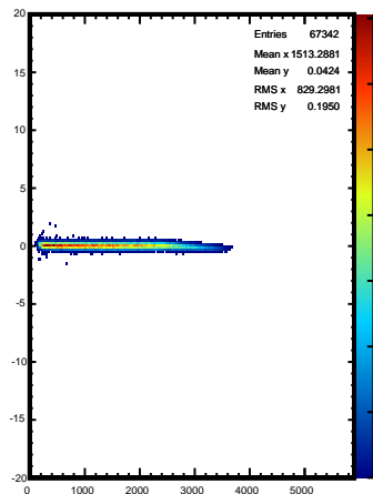
fDelta_Theta*180.0/TMath::Pi():fClusterEnergy
