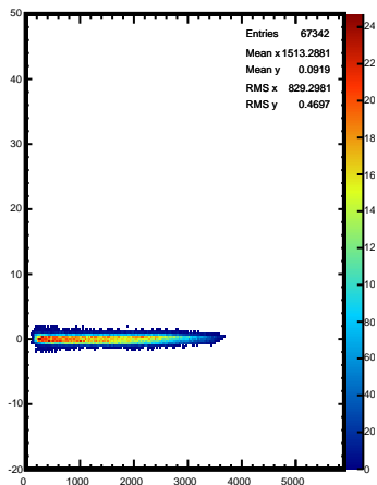
fDelta_Phi*180.0/TMath::Pi():fClusterEnergy
