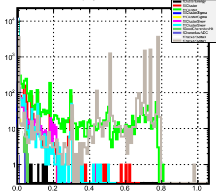
differences (impact of variables on ANN)
