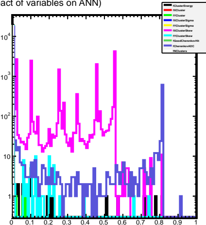
Impact of variables on ANN
