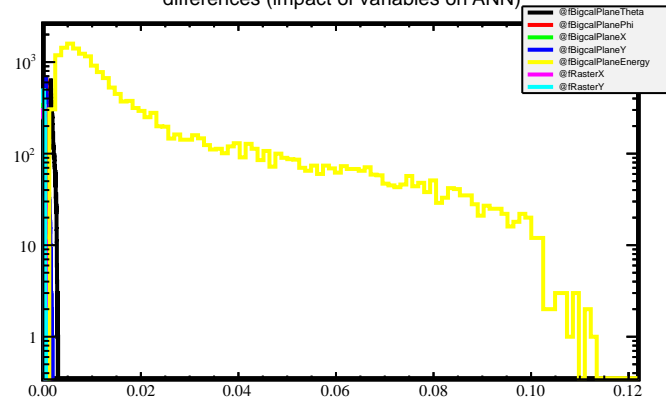
differences (impact of variables on ANN)
