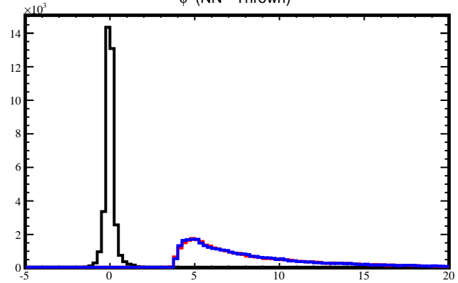
\phi (NN - Thrown)
