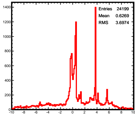
\theta Diff (NN - Thrown)
