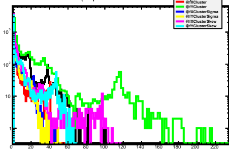
differences (impact of variables on \Delta )
