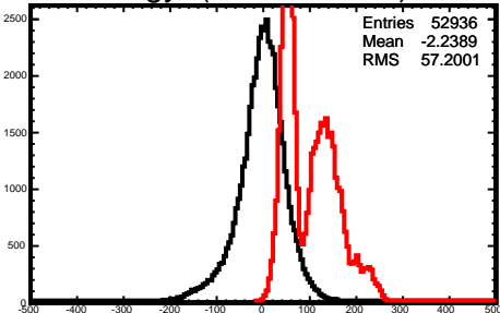
Energy (NN - Thrown)
