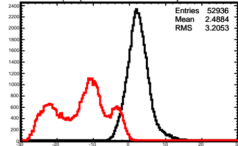
\phi (NN - Thrown)
