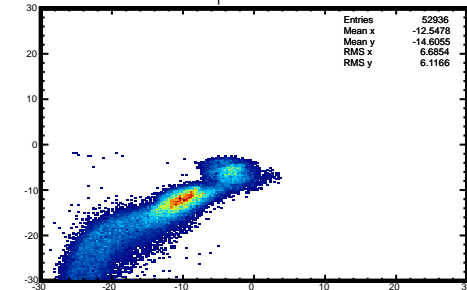
\Delta \phi test
