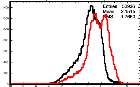
\theta (NN - Thrown)
