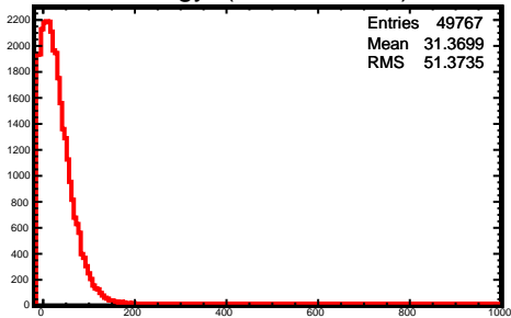
\Delta Energy (NN - Thrown)
