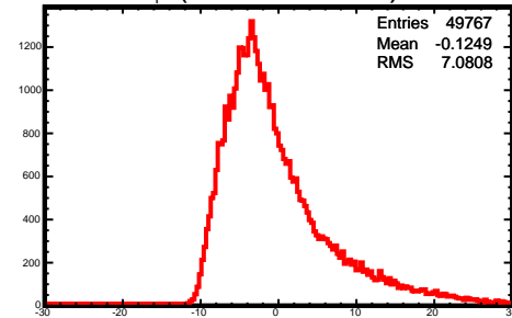
\Delta \phi (NN - Thrown)
