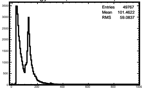
Energy Diff (NN - Thrown)
