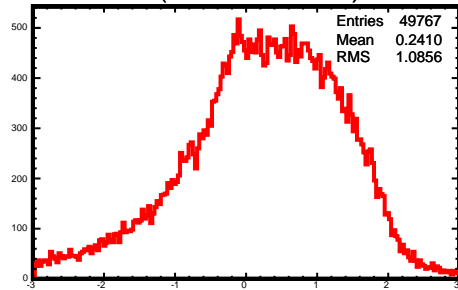
\Delta \theta (NN - Thrown)
