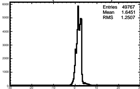
\theta Diff (NN - Thrown)
