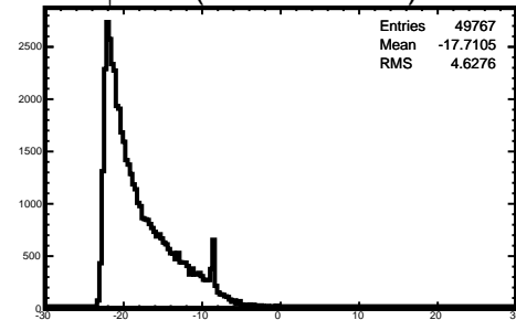
\phi Diff (NN - Thrown)
