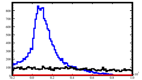
\Delta Energy (Thrown)
