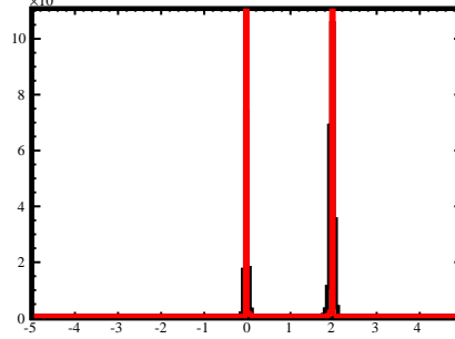
x (NN - Thrown)
