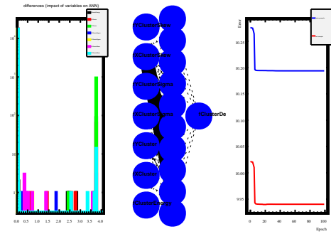
y (NN - Thrown)
