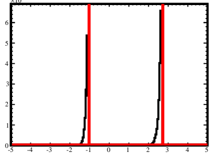
y (NN - Thrown)
