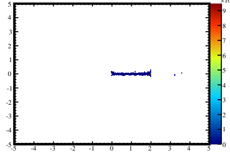
\Delta x test
