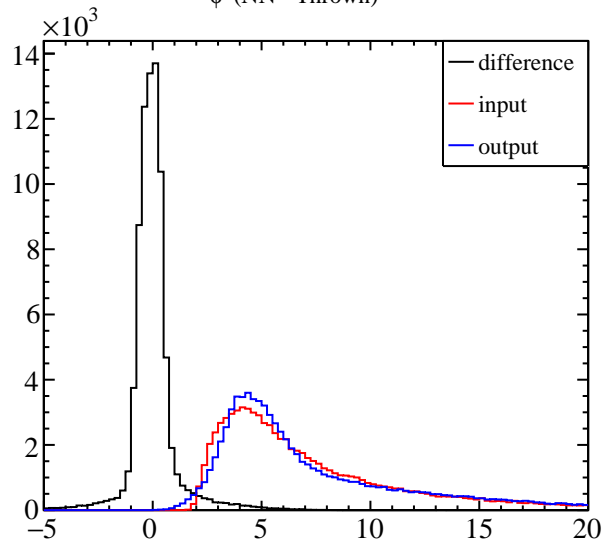
\phi (NN - Thrown)
