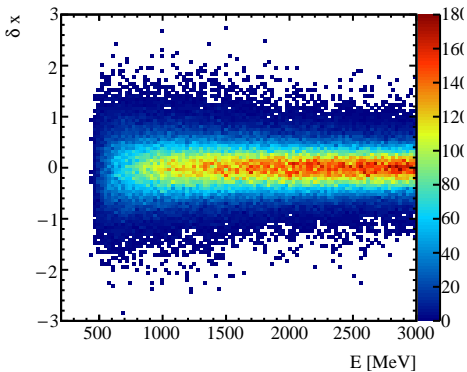
\delta x vs Energy
