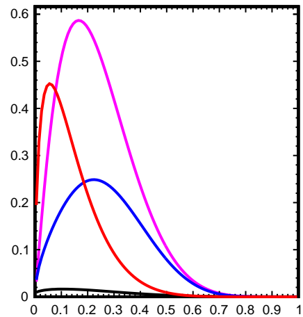
\Delta g(x)
