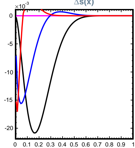
\Delta s(x)
