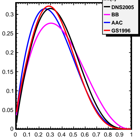
\Delta u(x)
