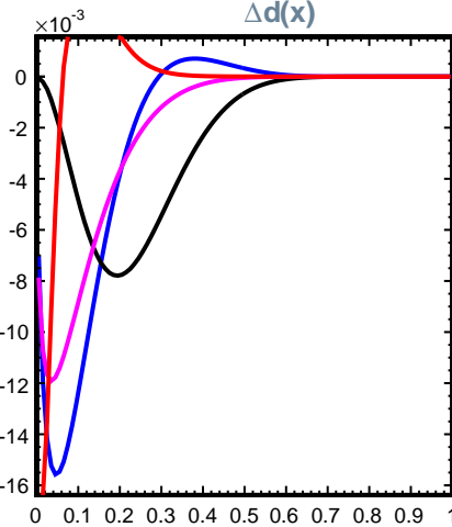
\Delta \bar{d}(x)
