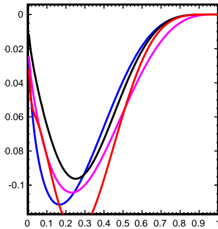
\Delta d(x)
