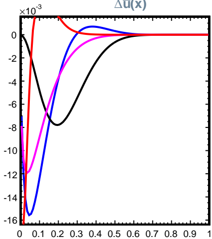
\Delta \bar{u}(x)
