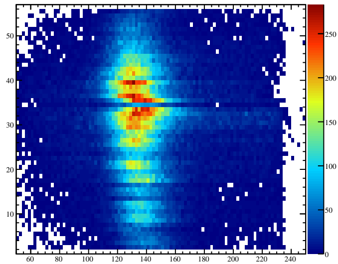
YvsMass-0
