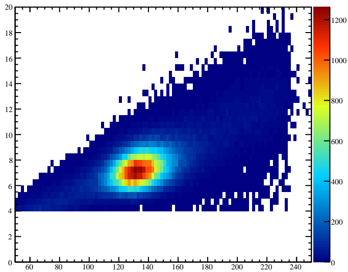
AnglevsMass-0
