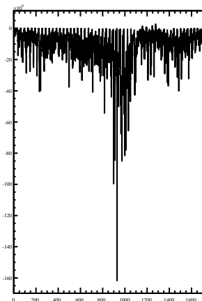
D Vector
