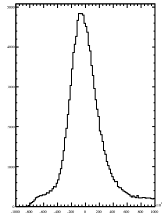
fMassBiasHist
