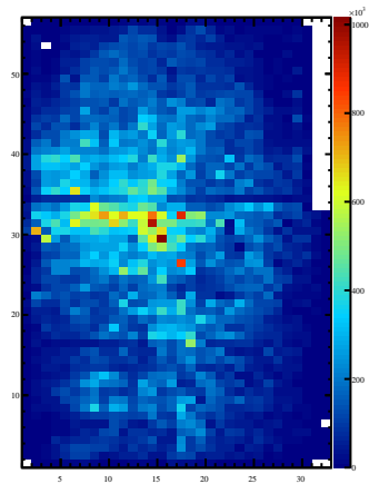
Bigcal P0 Event Clusters
