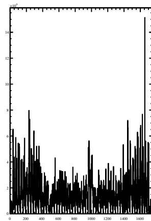
L Vector
