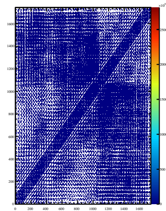
C matrix
