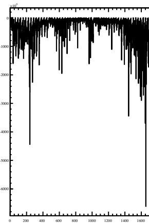
D Vector
