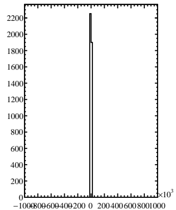
fMassBiasHist
