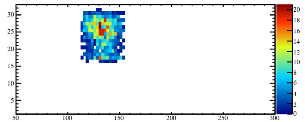
Mass vs x-9
